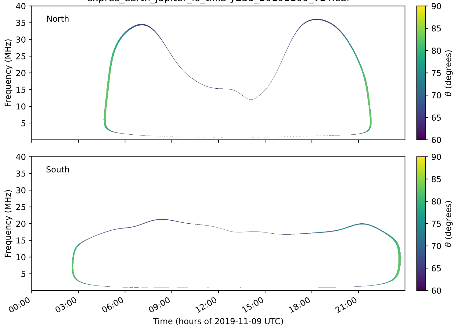
expres_earth_jupiter_io_txka-y235_20191109_v14.cdf
