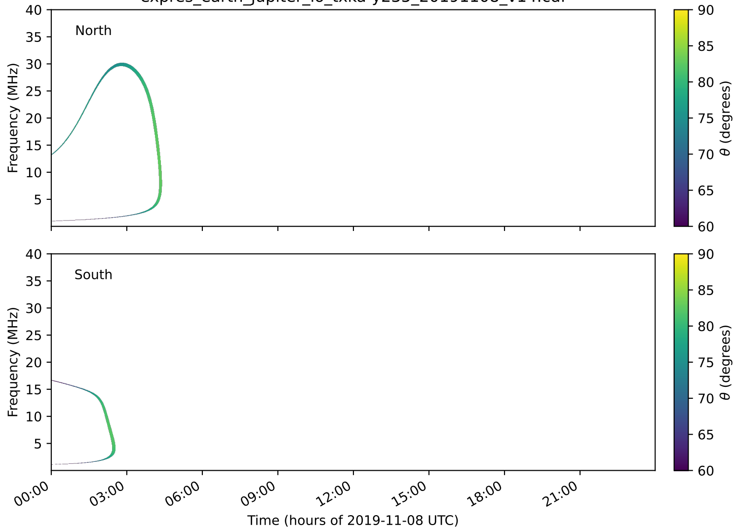
expres_earth_jupiter_io_txka-y235_20191108_v14.cdf
