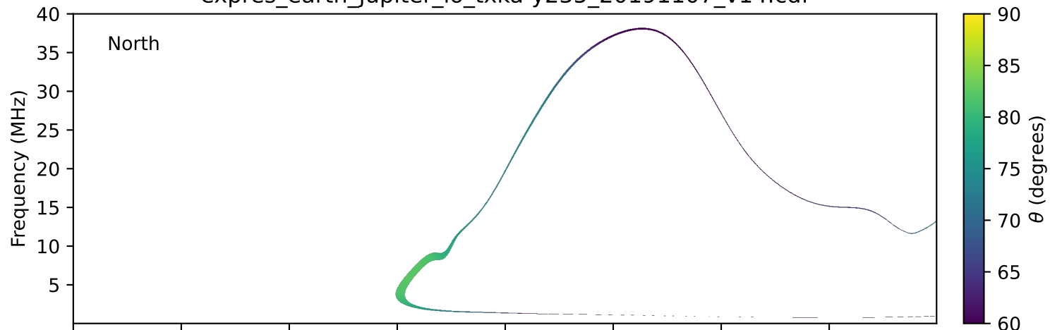
expres_earth_jupiter_io_txka-y235_20191107_v14.cdf
