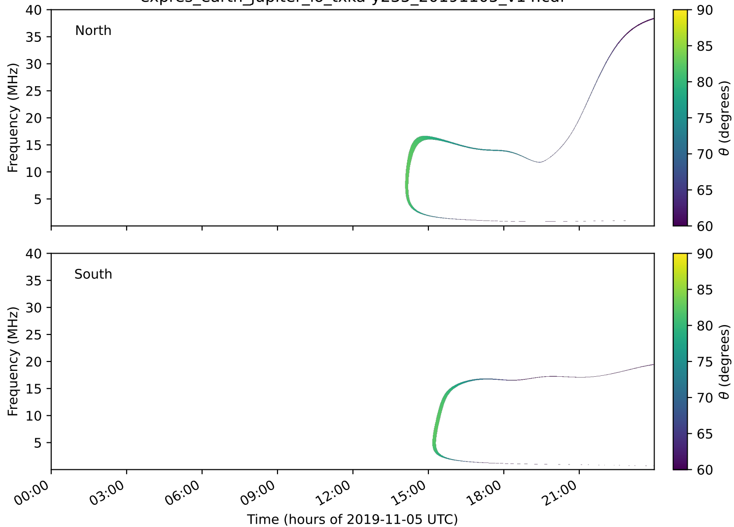
expres_earth_jupiter_io_txka-y235_20191105_v14.cdf
