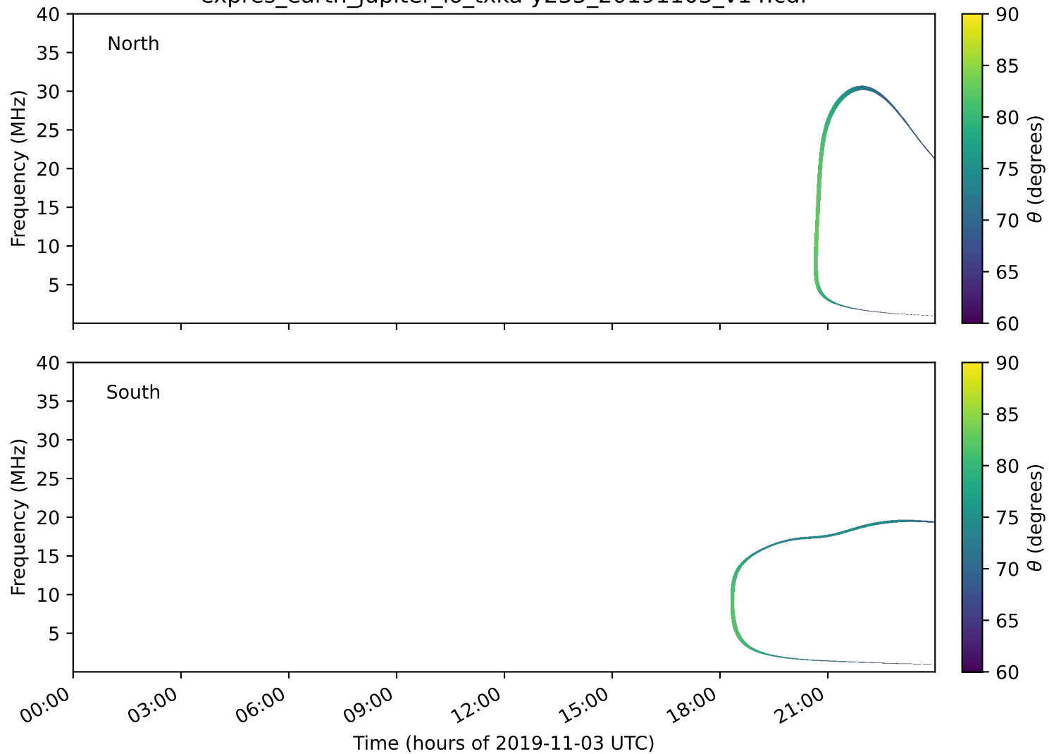
expres_earth_jupiter_io_txka-y235_20191103_v14.cdf
