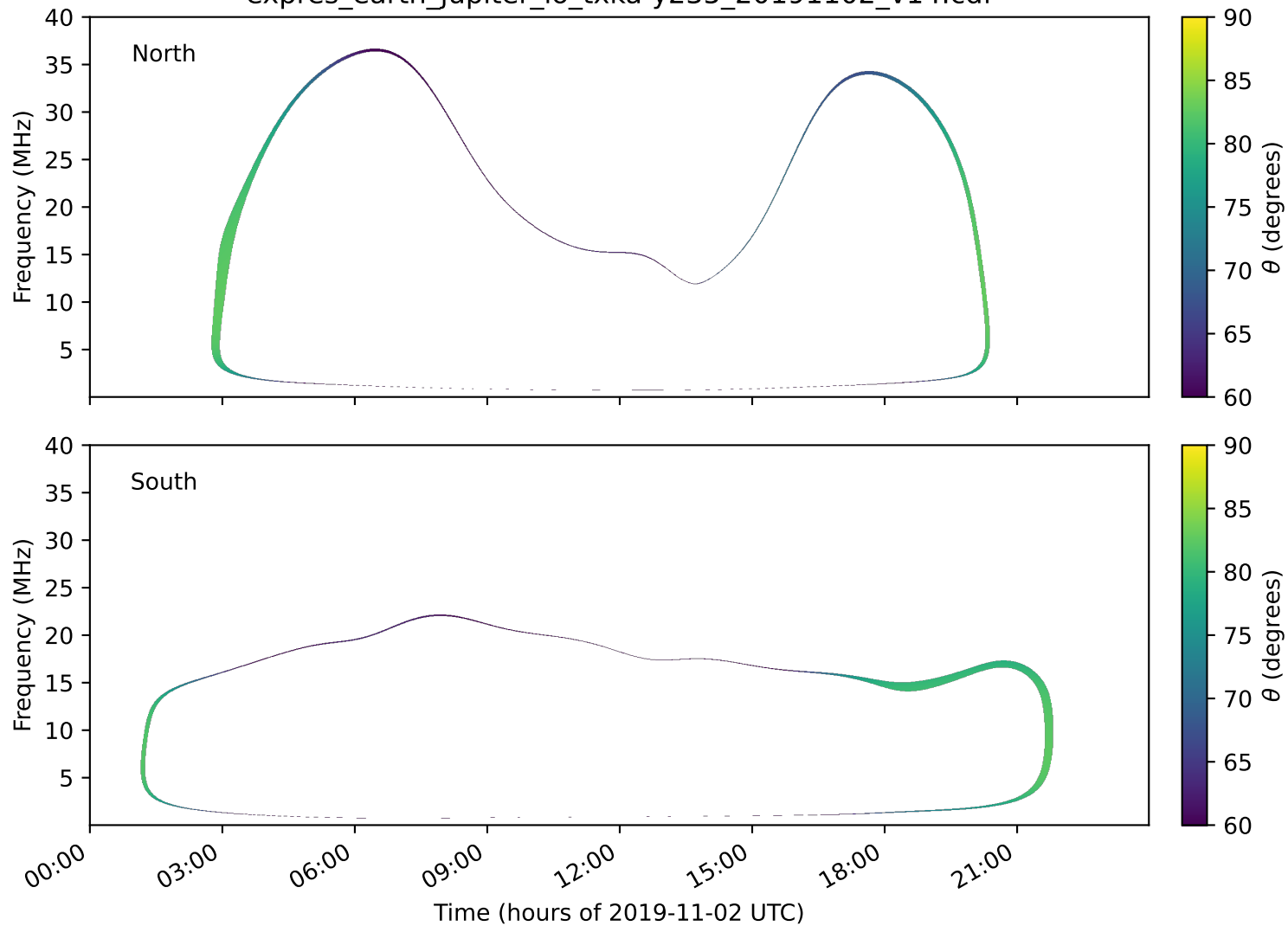
expres_earth_jupiter_io_txka-y235_20191102_v14.cdf
