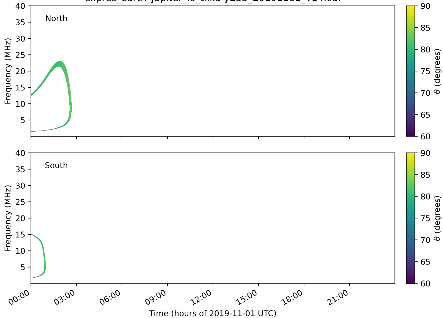
expres_earth_jupiter_io_txka-y235_20191101_v14.cdf
