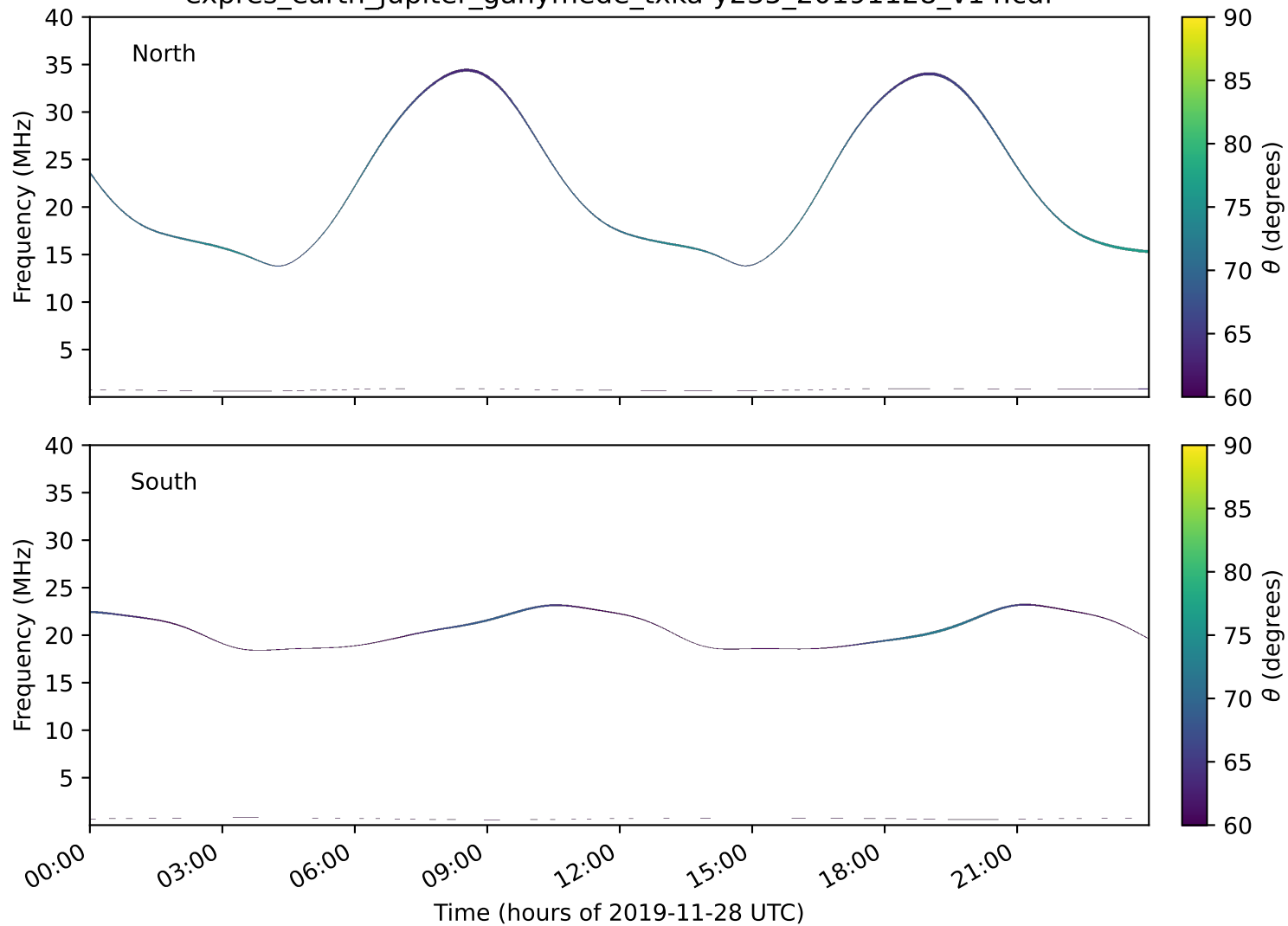
expres_earth_jupiter_ganymede_txka-y235_20191128_v14.cdf
