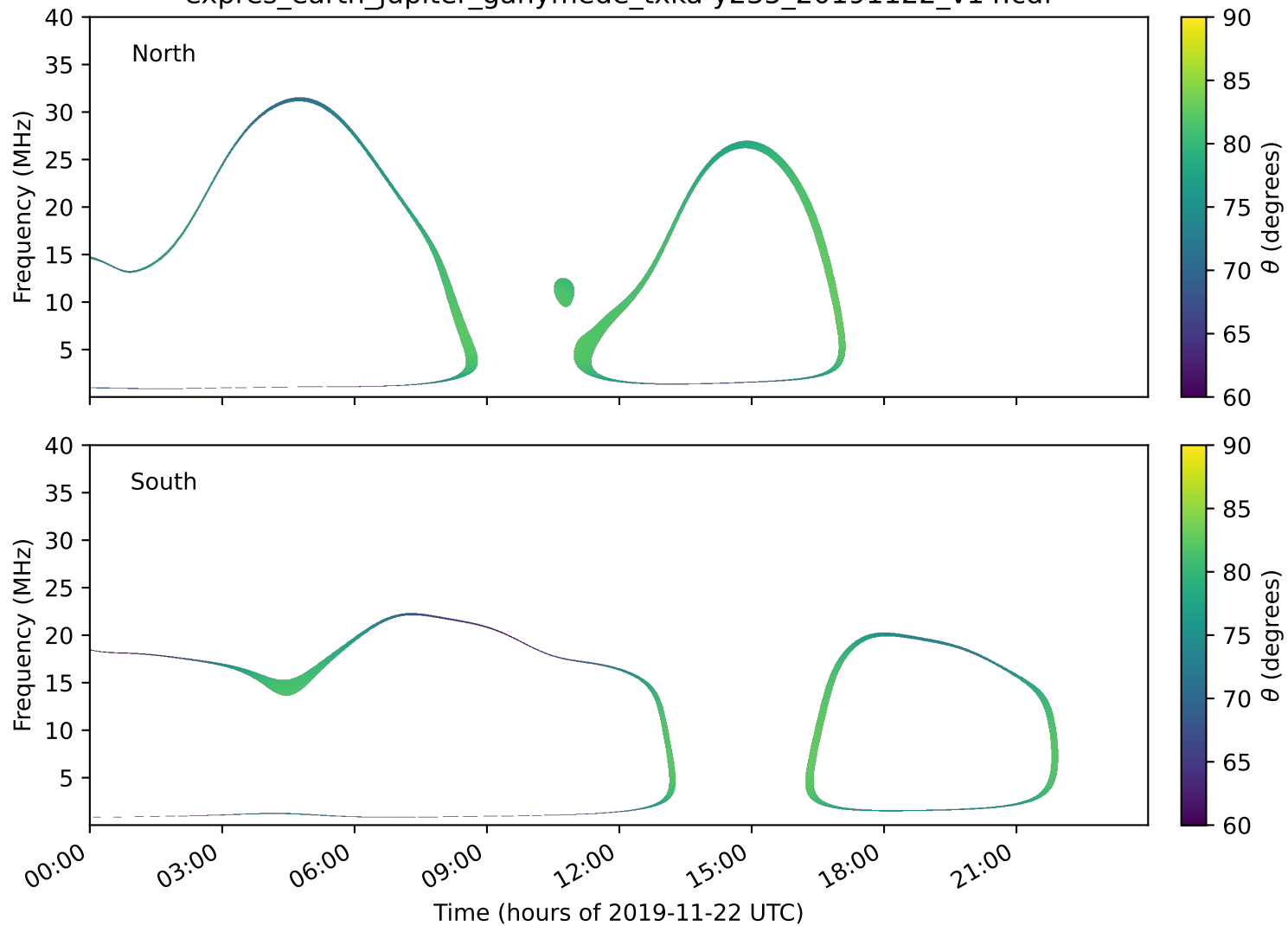
expres_earth_jupiter_ganymede_txka-y235_20191122_v14.cdf
