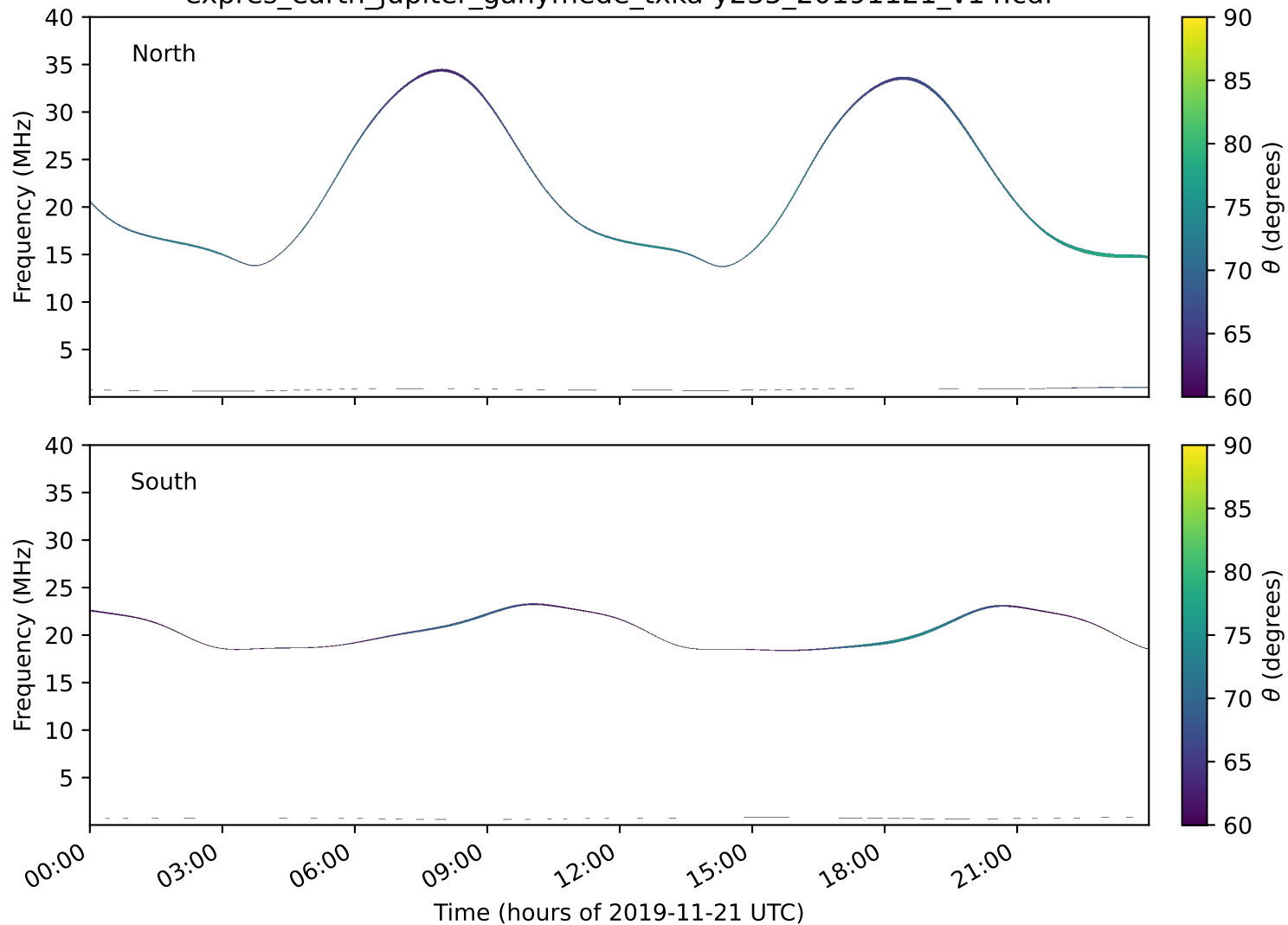
expres_earth_jupiter_ganymede_txka-y235_20191121_v14.cdf
