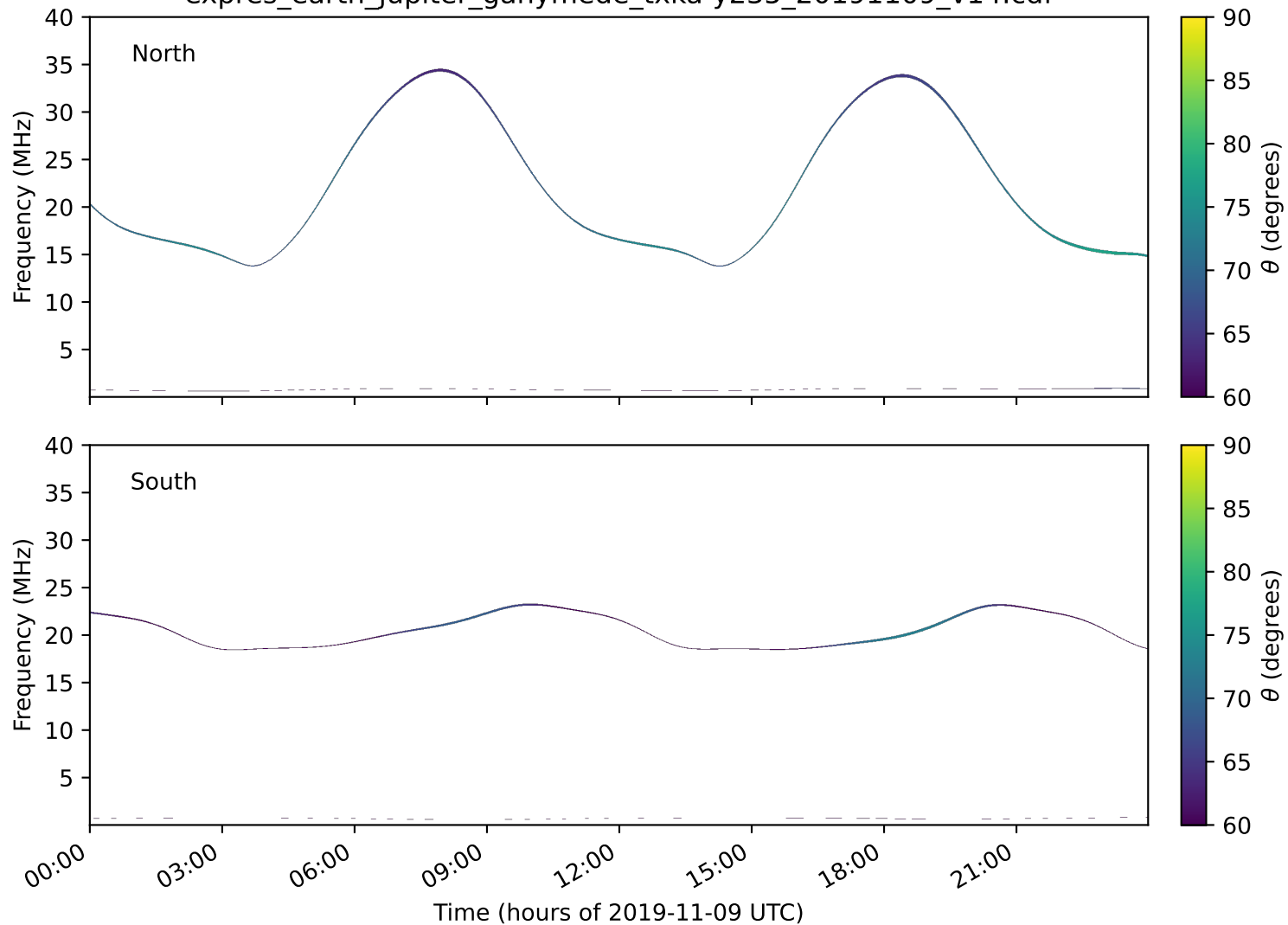
expres_earth_jupiter_ganymede_txka-y235_20191109_v14.cdf
