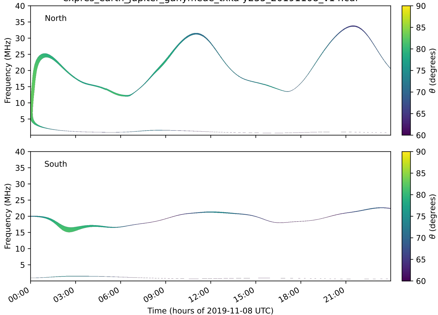
expres_earth_jupiter_ganymede_txka-y235_20191108_v14.cdf
