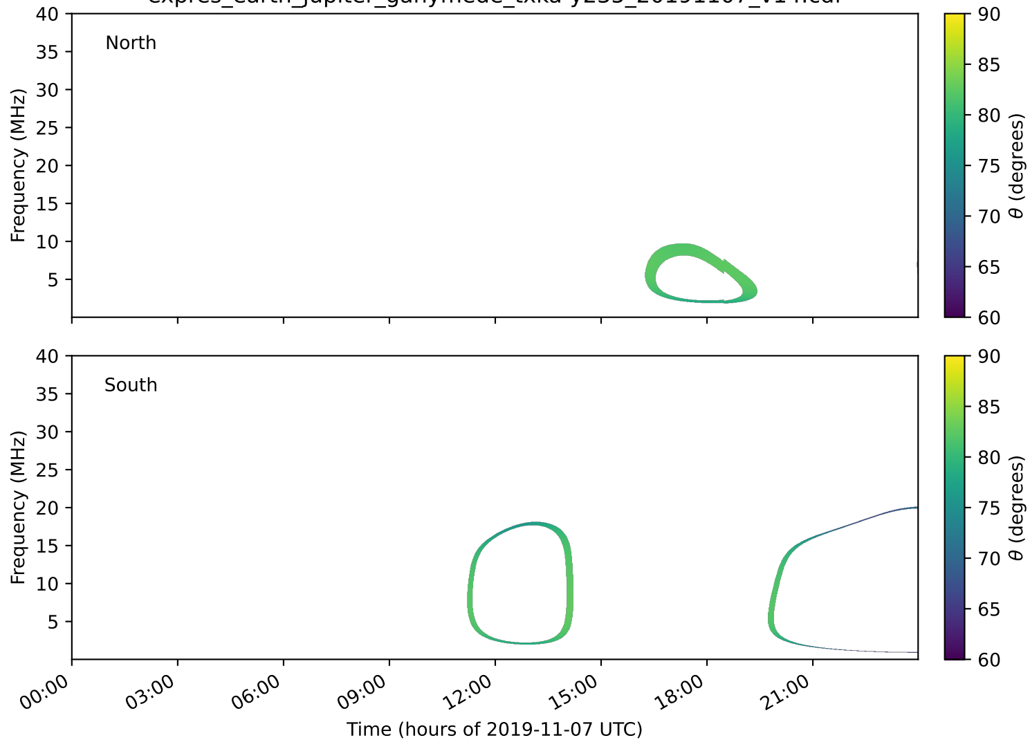
expres_earth_jupiter_ganymede_txka-y235_20191107_v14.cdf
