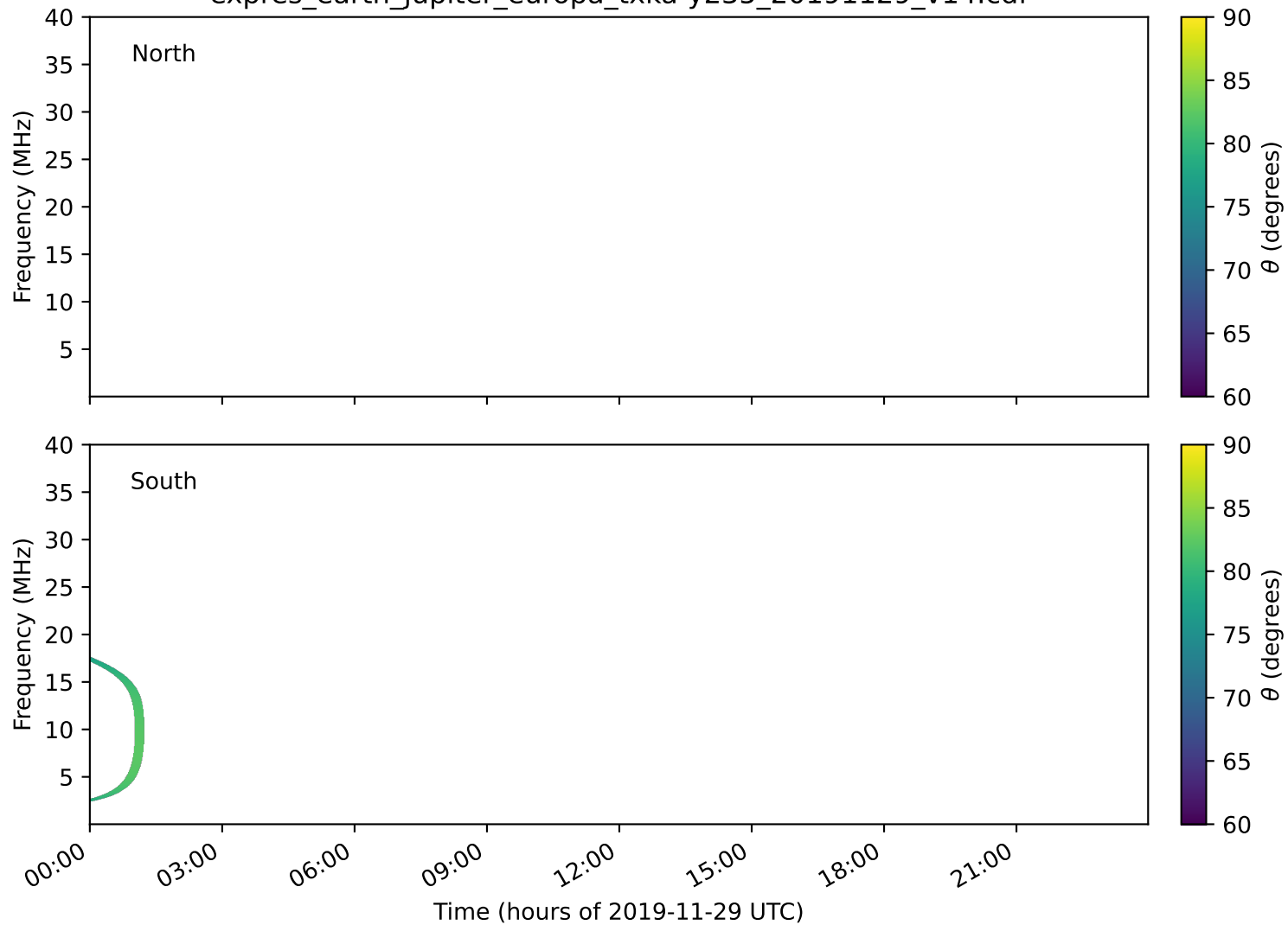
expres_earth_jupiter_europa_txka-y235_20191129_v14.cdf
