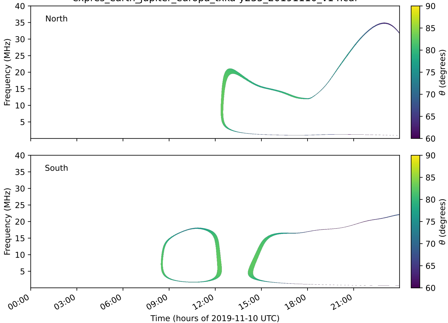
expres_earth_jupiter_europa_txka-y235_20191110_v14.cdf
