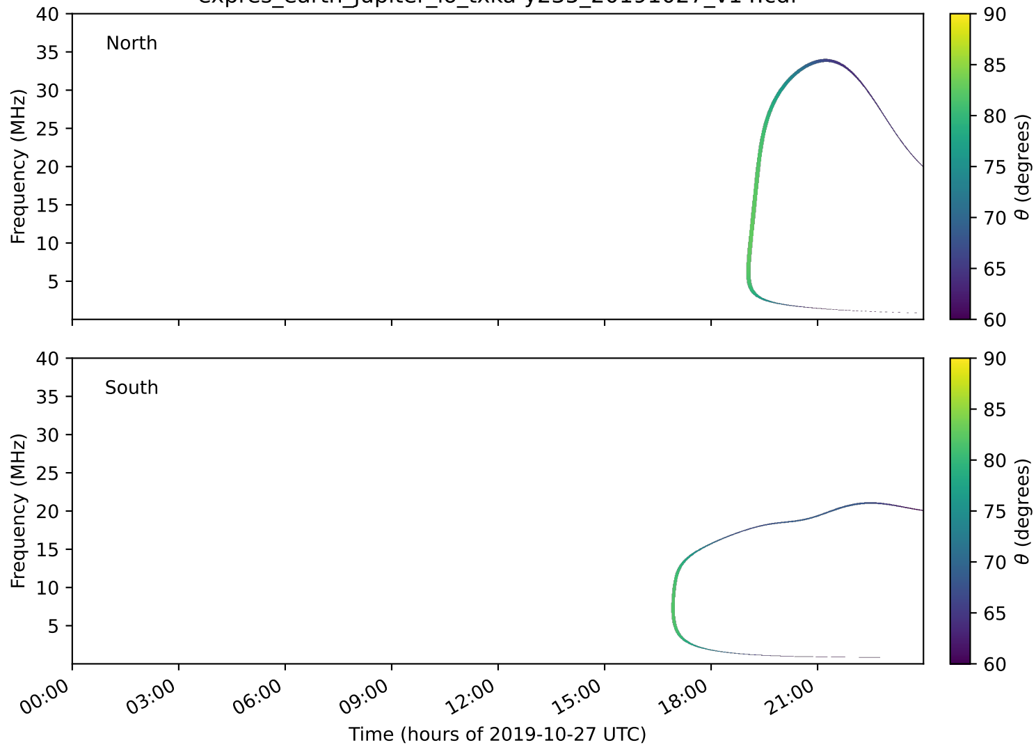
expres_earth_jupiter_io_txka-y235_20191027_v14.cdf
