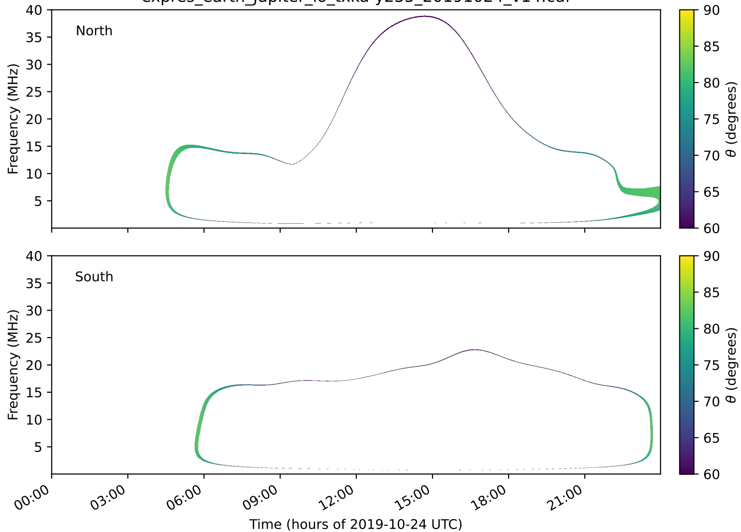
expres_earth_jupiter_io_txka-y235_20191024_v14.cdf
