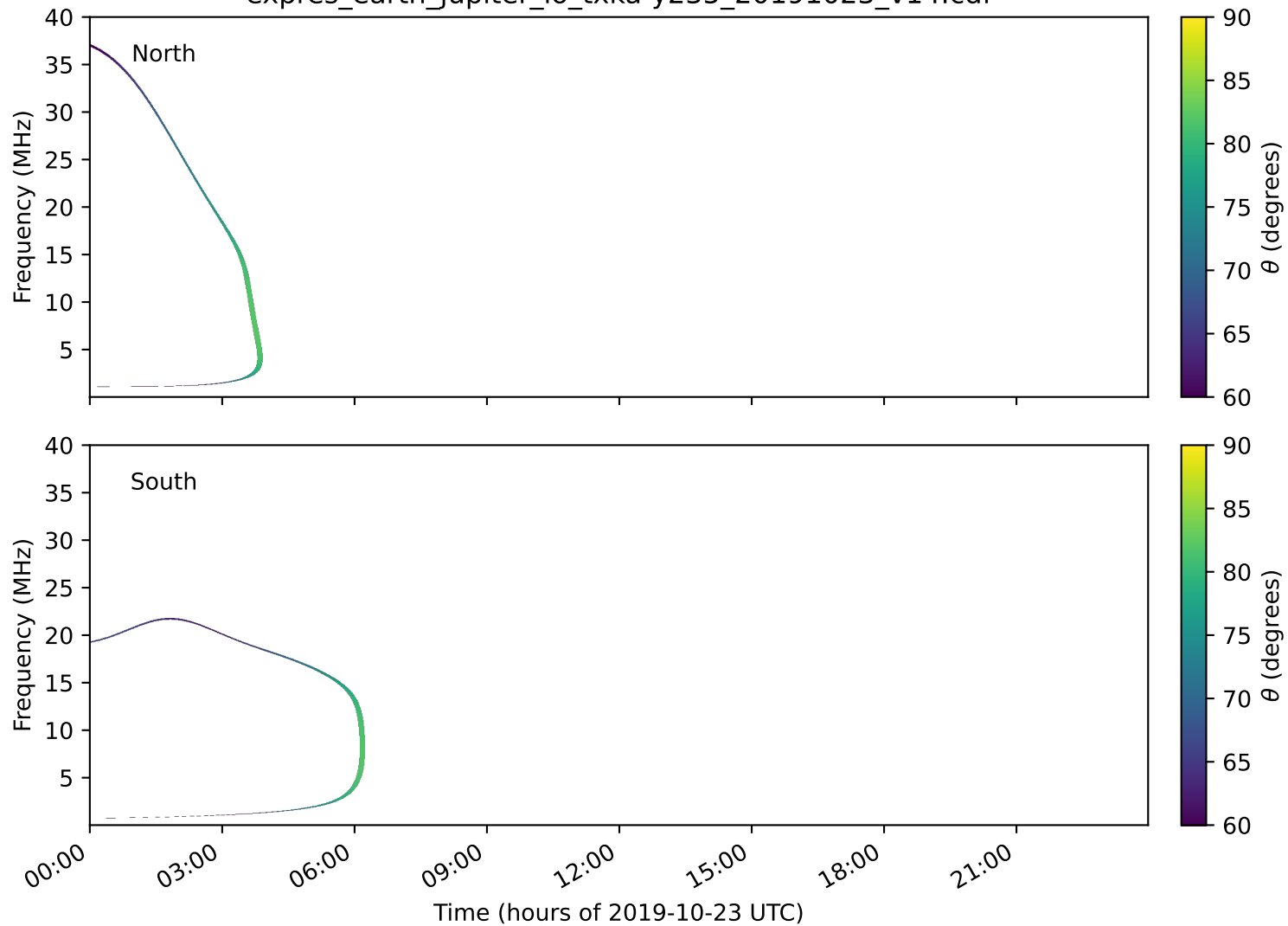
expres_earth_jupiter_io_txka-y235_20191023_v14.cdf
