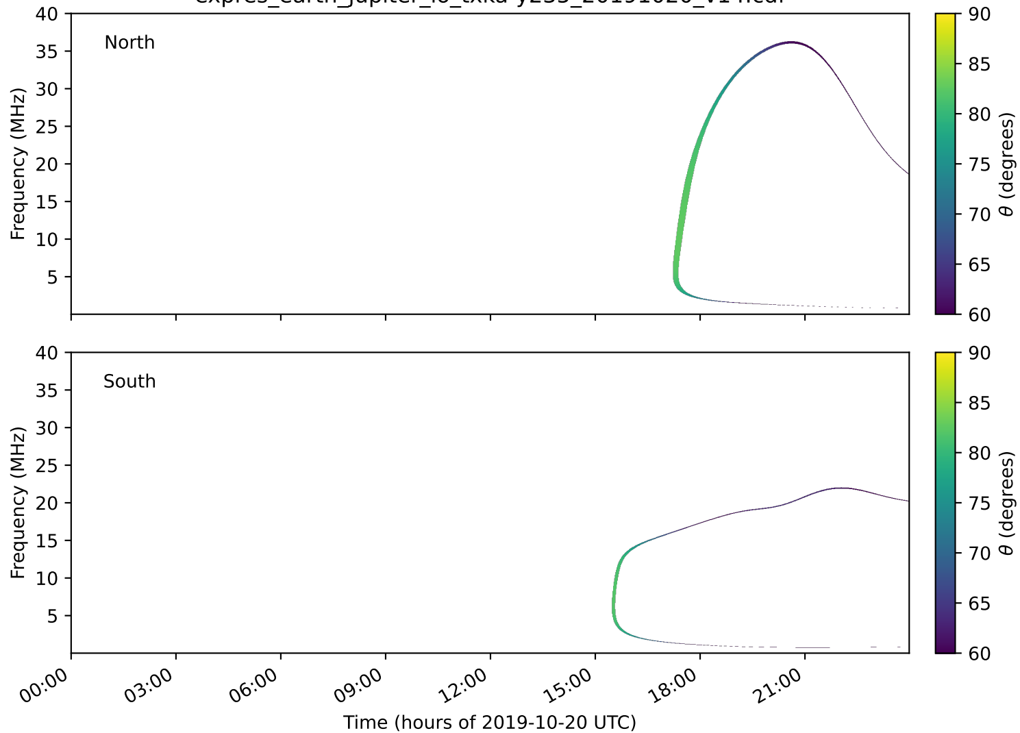
expres_earth_jupiter_io_txka-y235_20191020_v14.cdf
