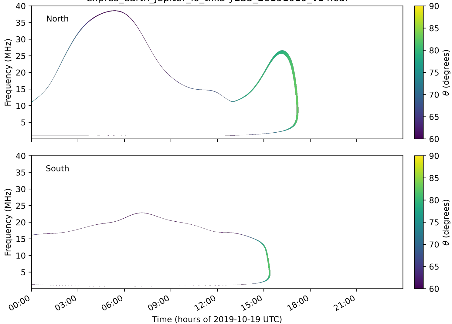
expres_earth_jupiter_io_txka-y235_20191019_v14.cdf
