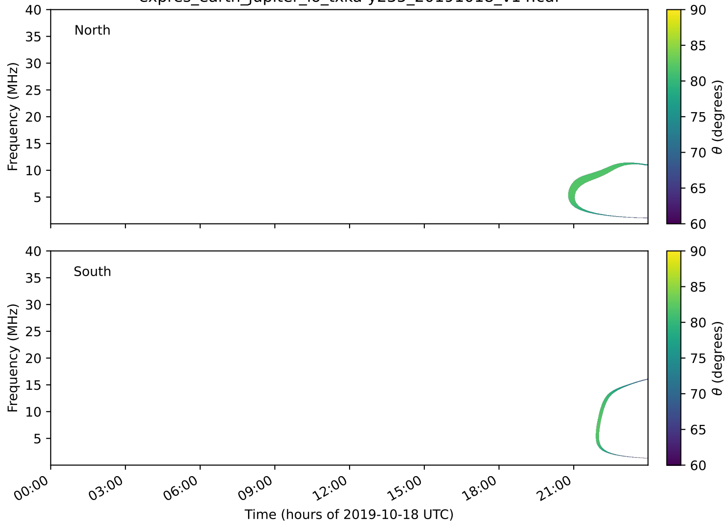
expres_earth_jupiter_io_txka-y235_20191018_v14.cdf
