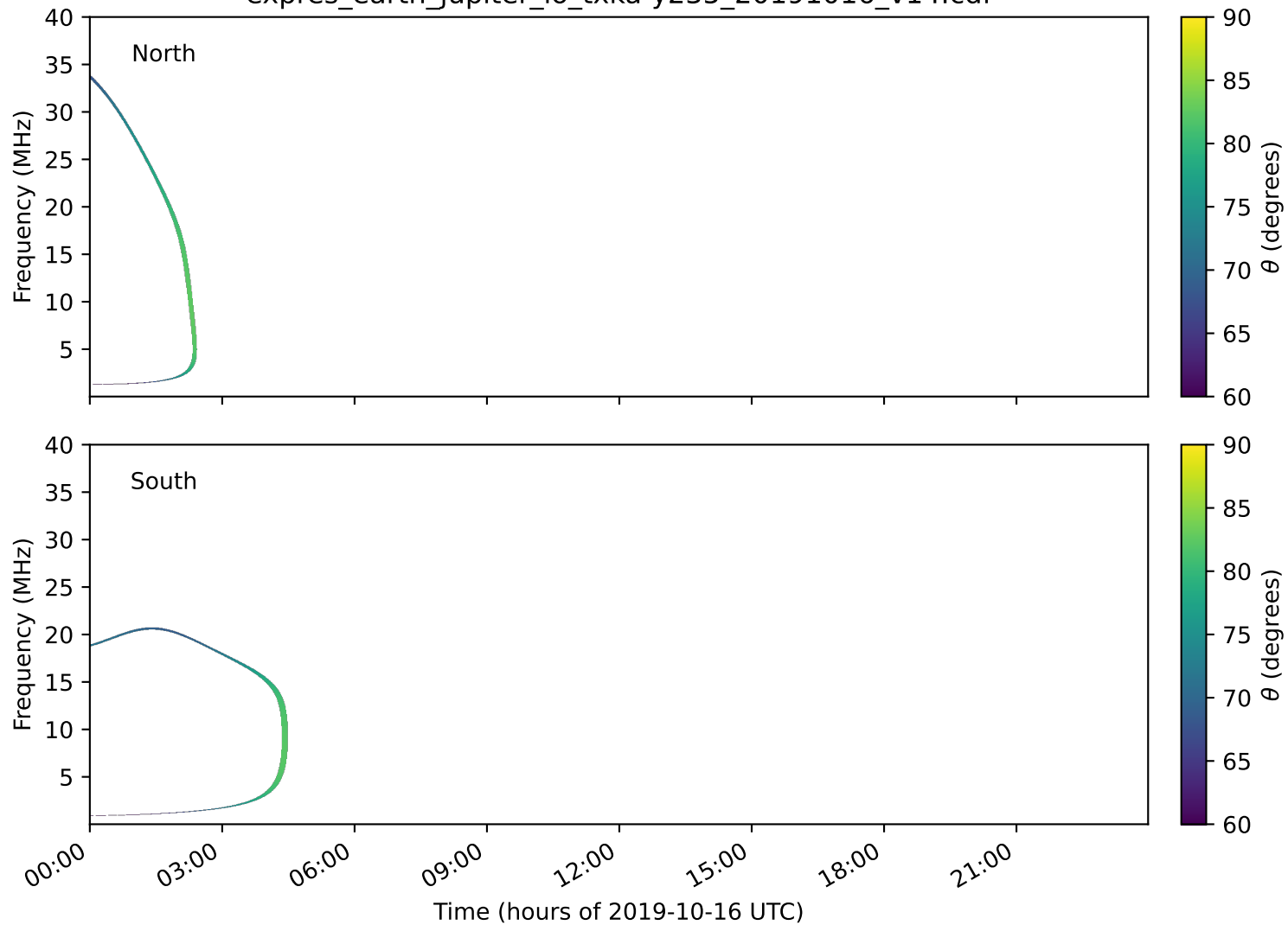
expres_earth_jupiter_io_txka-y235_20191016_v14.cdf
