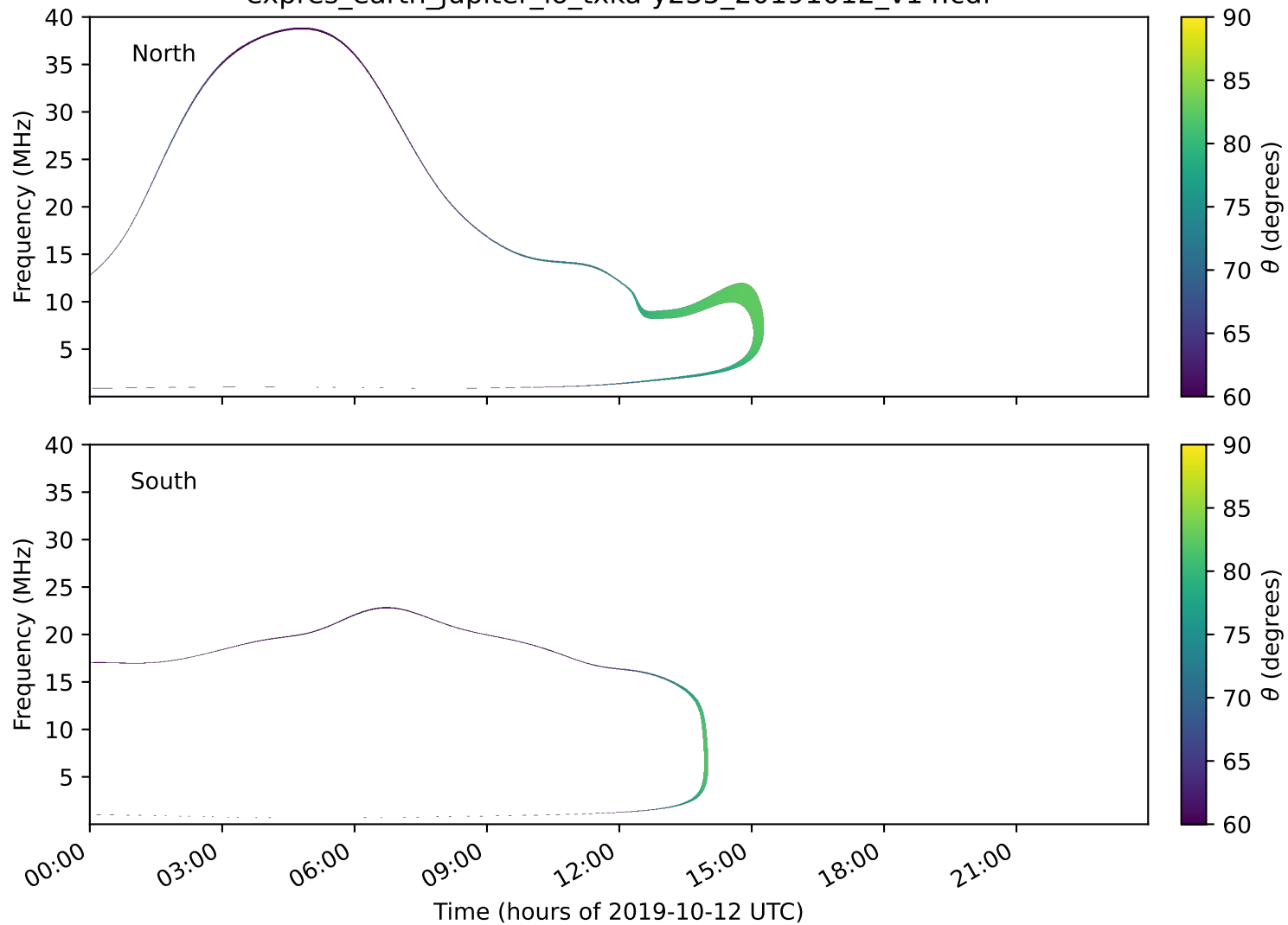
expres_earth_jupiter_io_txka-y235_20191012_v14.cdf
