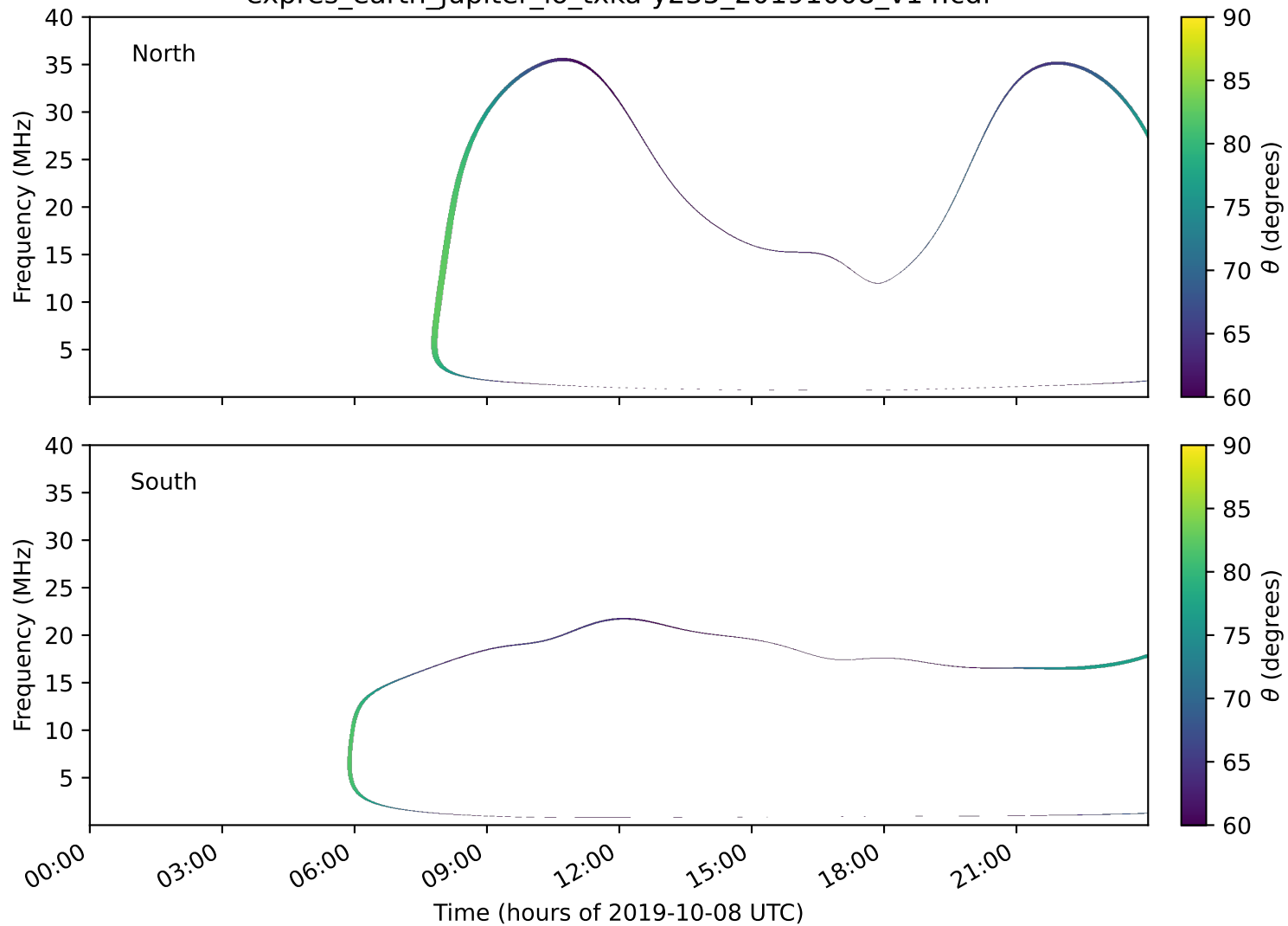
expres_earth_jupiter_io_txka-y235_20191008_v14.cdf
