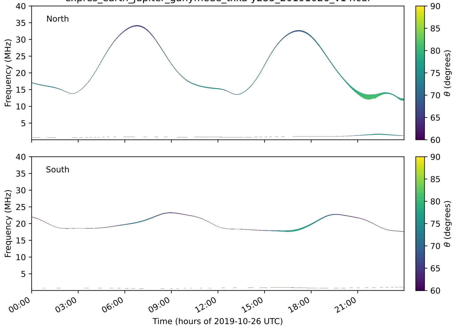
expres_earth_jupiter_ganymede_txka-y235_20191026_v14.cdf
