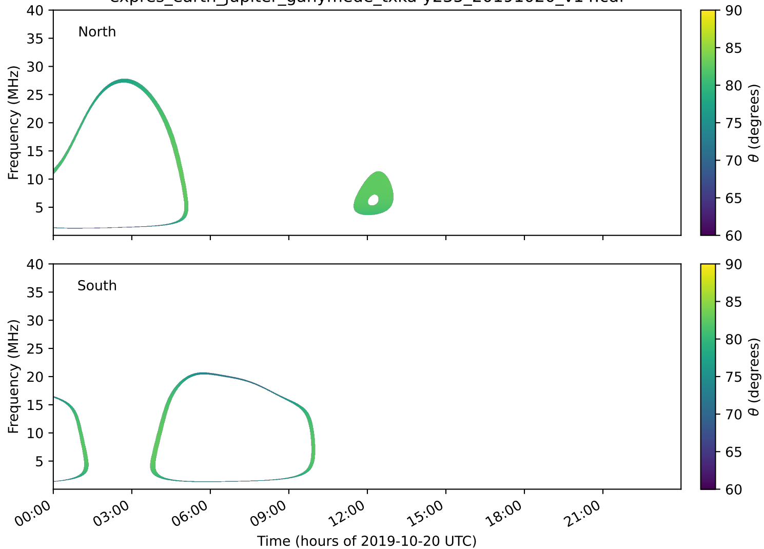
expres_earth_jupiter_ganymede_txka-y235_20191020_v14.cdf
