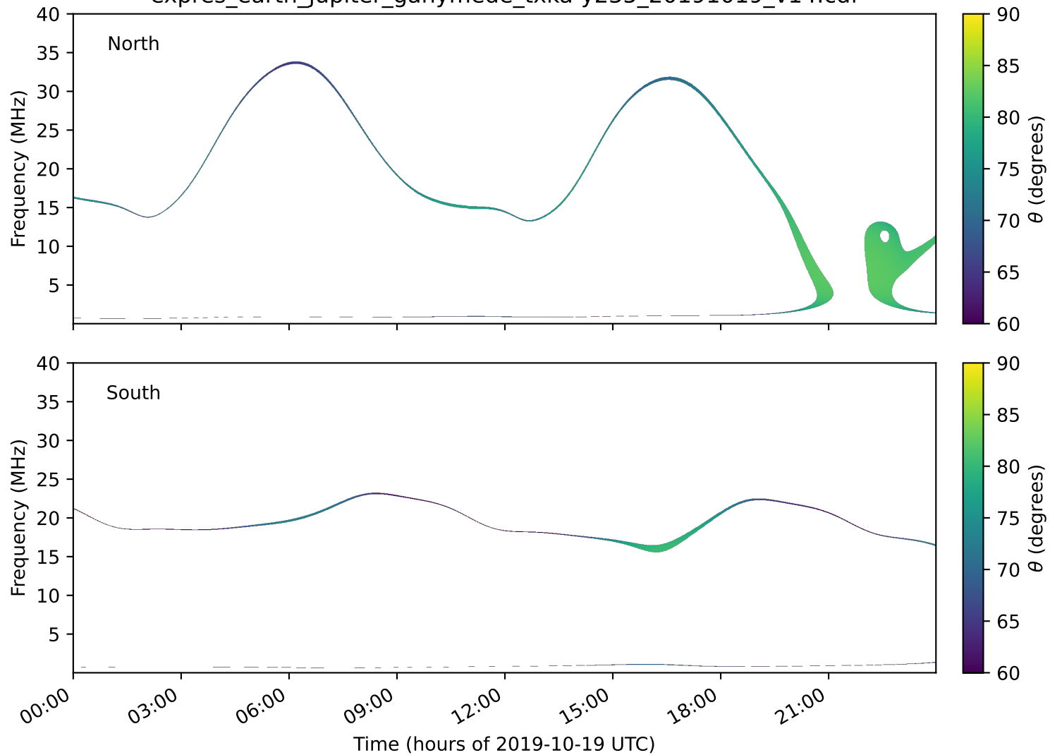
expres_earth_jupiter_ganymede_txka-y235_20191019_v14.cdf
