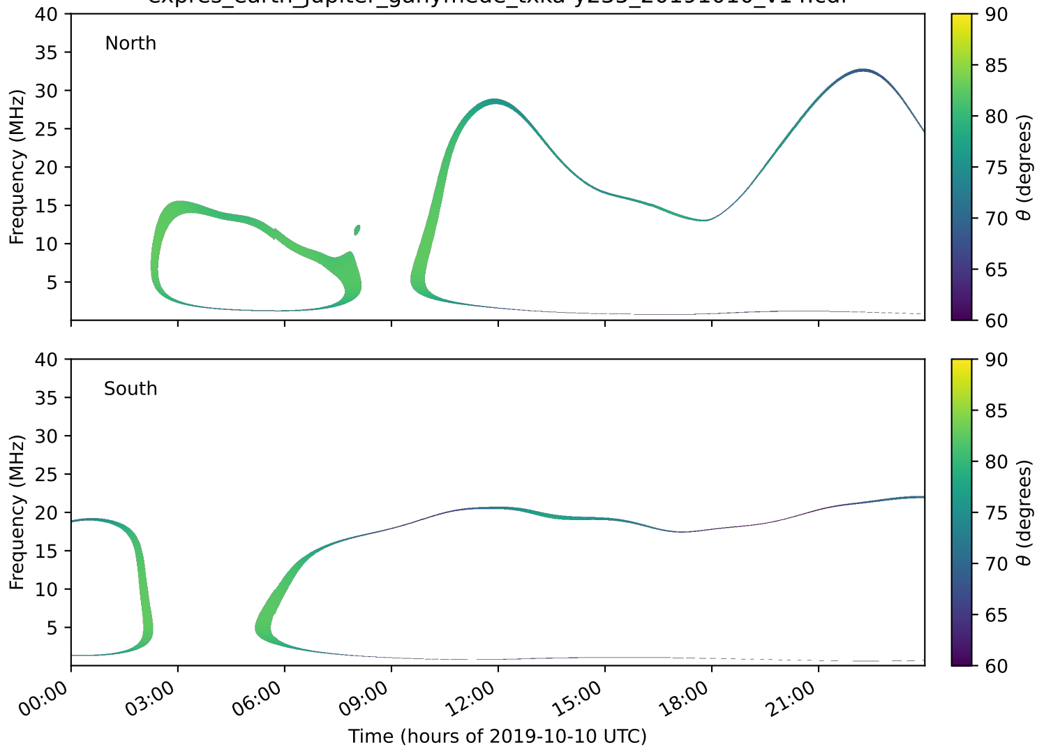
expres_earth_jupiter_ganymede_txka-y235_20191010_v14.cdf
