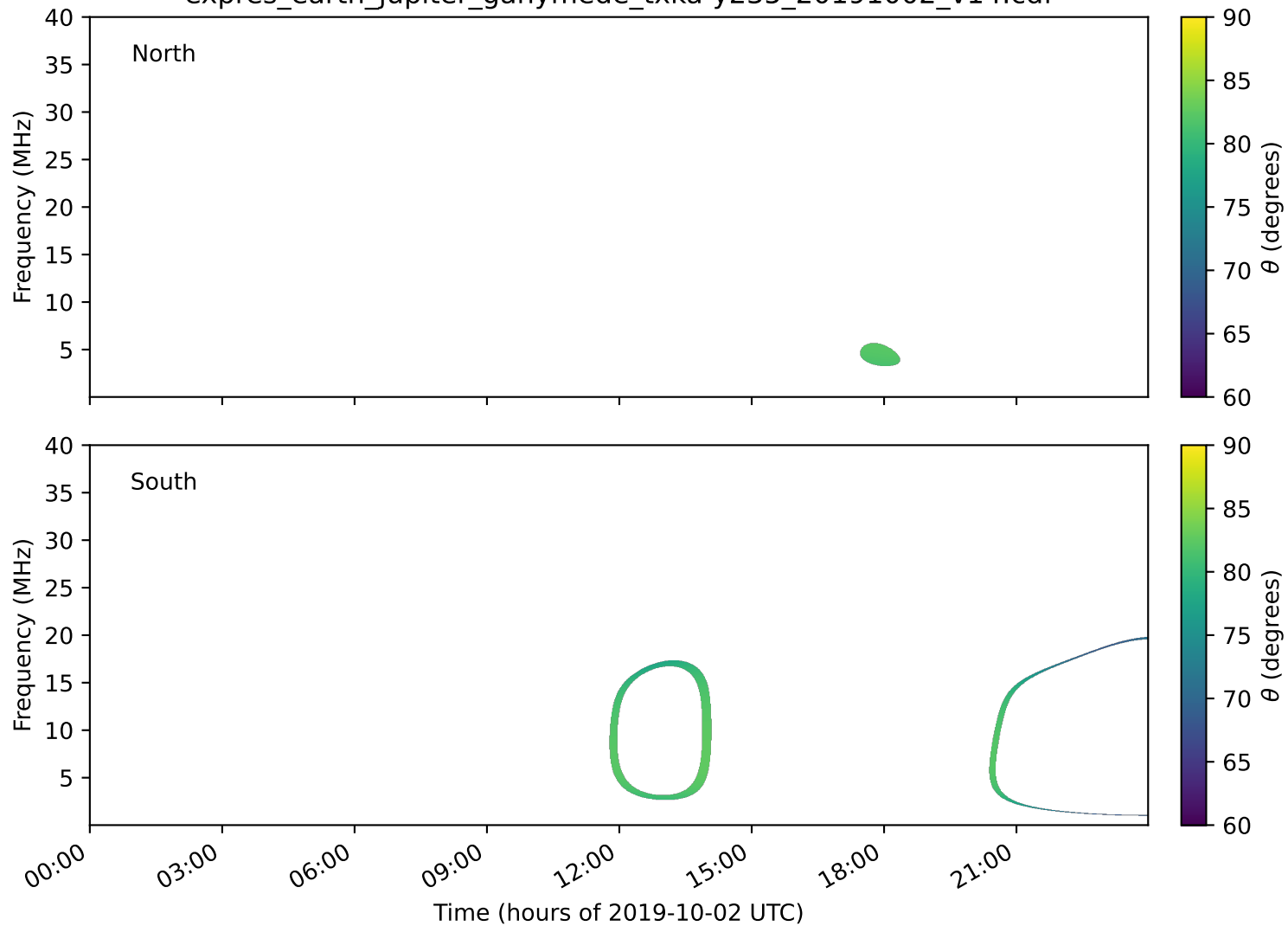
expres_earth_jupiter_ganymede_txka-y235_20191002_v14.cdf
