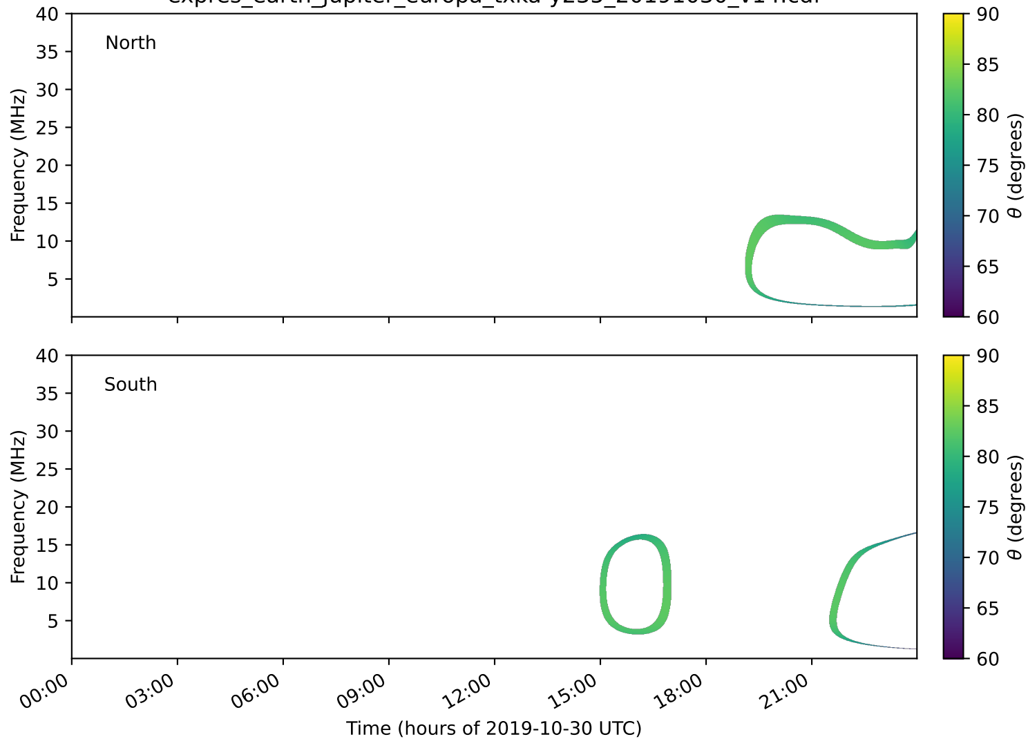
expres_earth_jupiter_europa_txka-y235_20191030_v14.cdf
