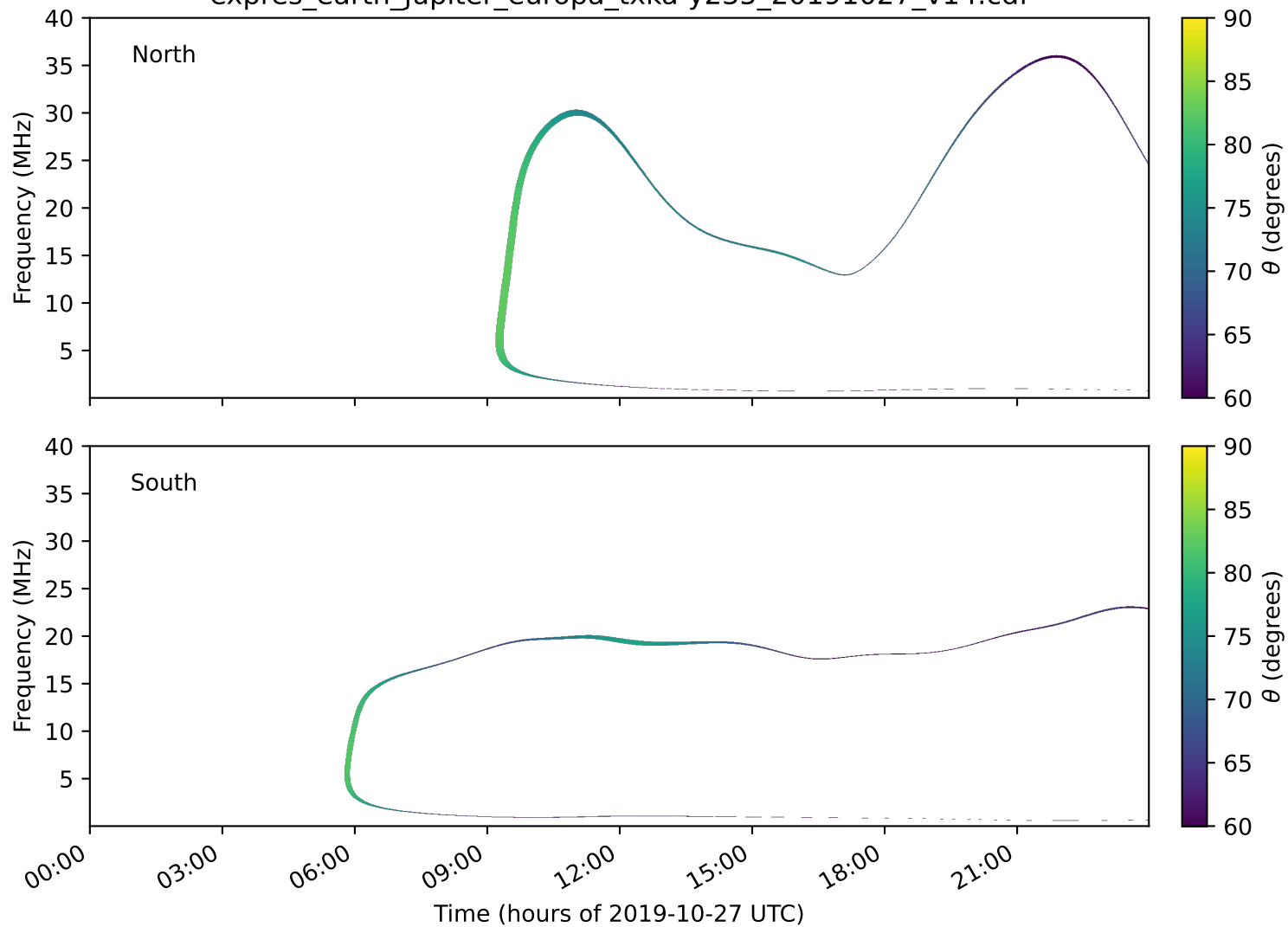
expres_earth_jupiter_europa_txka-y235_20191027_v14.cdf
