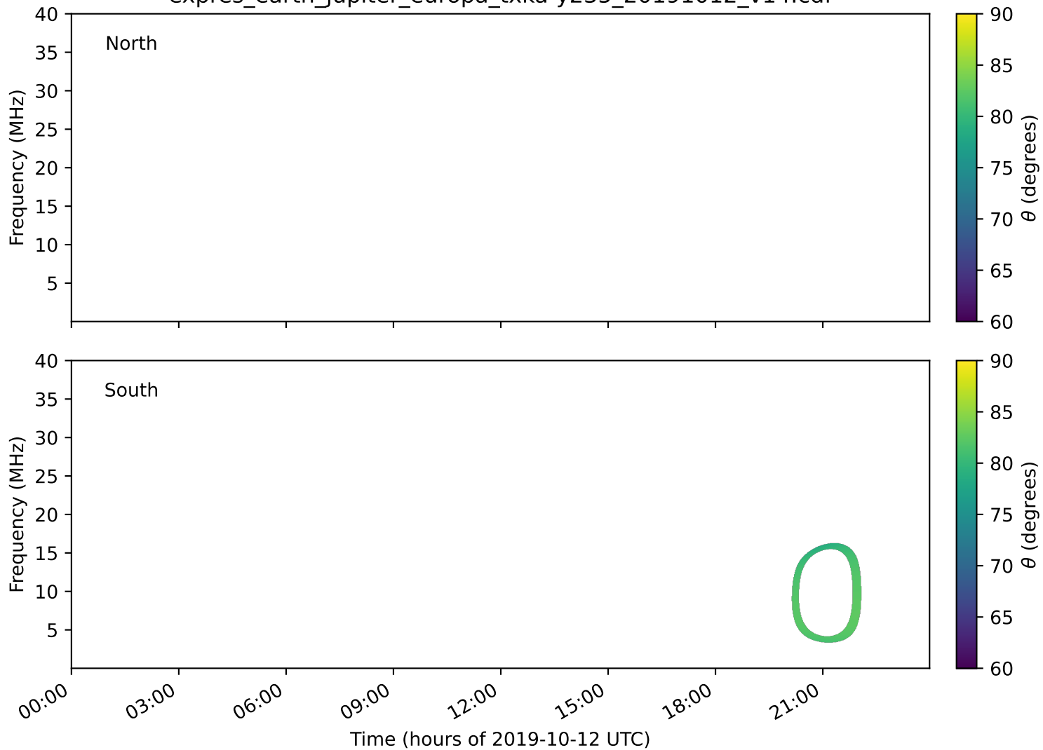
expres_earth_jupiter_europa_txka-y235_20191012_v14.cdf
