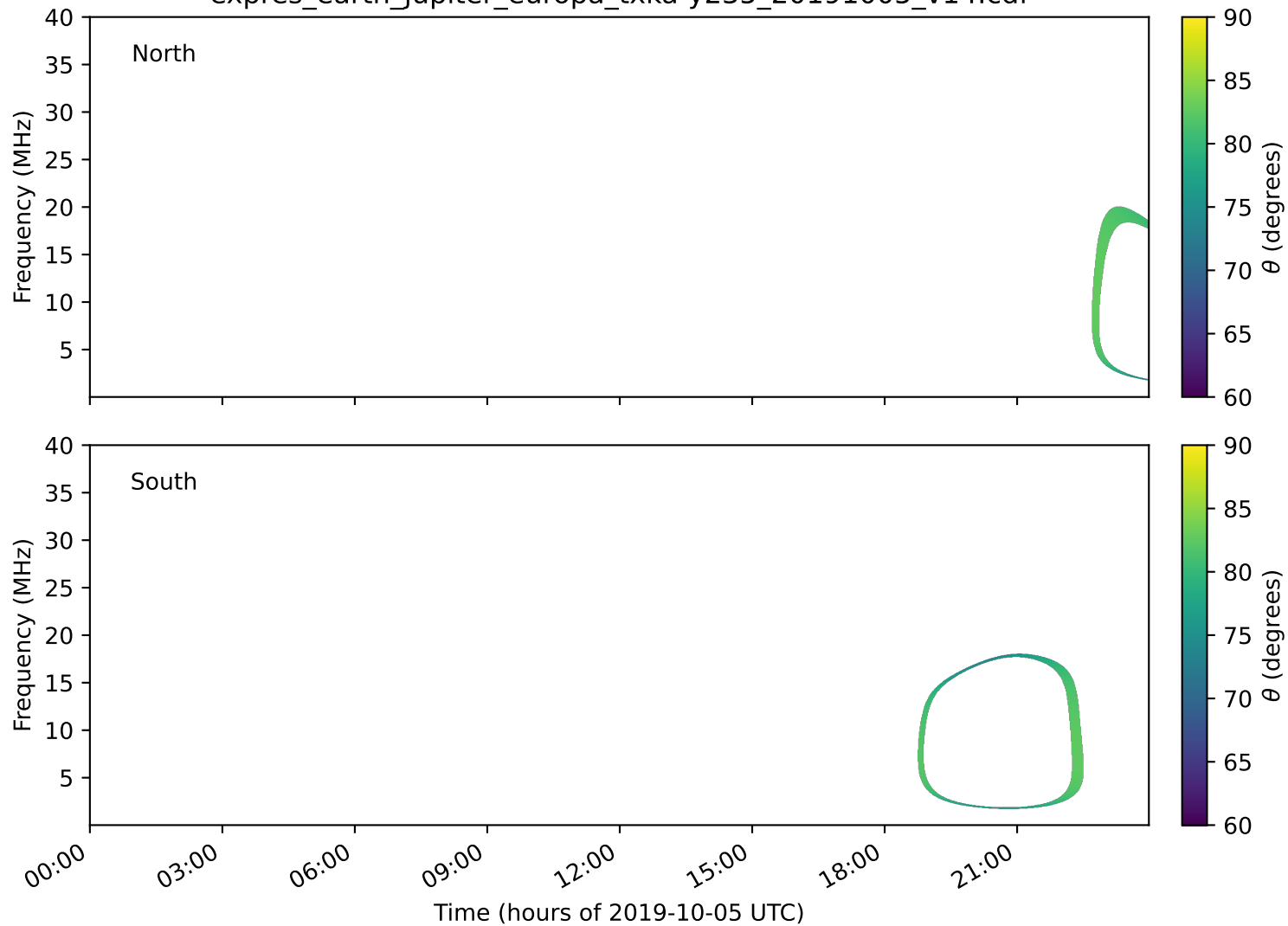
expres_earth_jupiter_europa_txka-y235_20191005_v14.cdf
