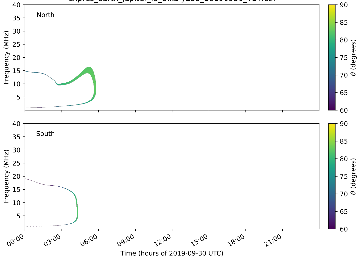
expres_earth_jupiter_io_txka-y235_20190930_v14.cdf
