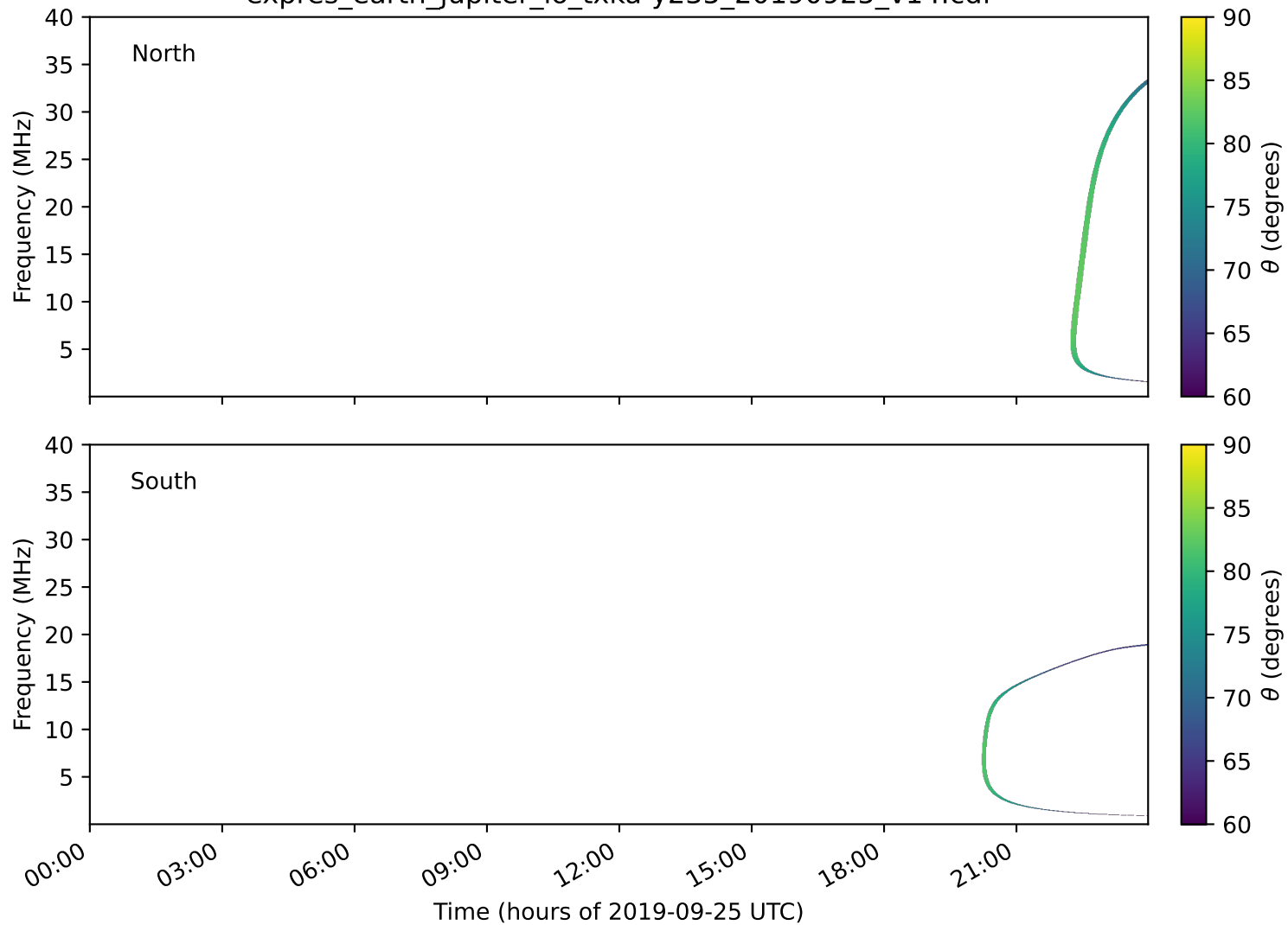
expres_earth_jupiter_io_txka-y235_20190925_v14.cdf
