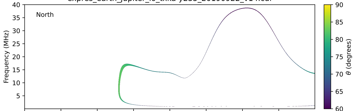
expres_earth_jupiter_io_txka-y235_20190922_v14.cdf
