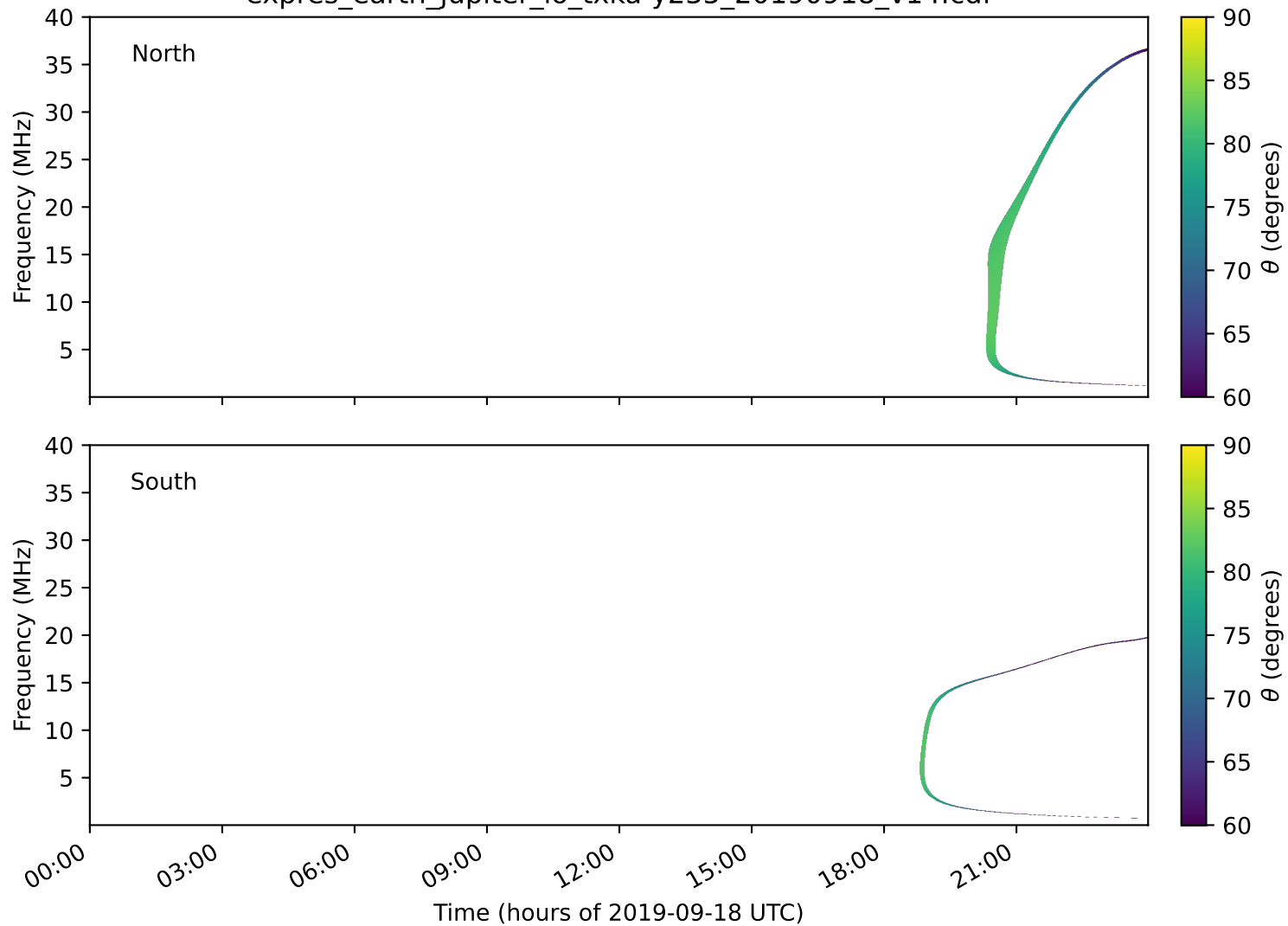
expres_earth_jupiter_io_txka-y235_20190918_v14.cdf
