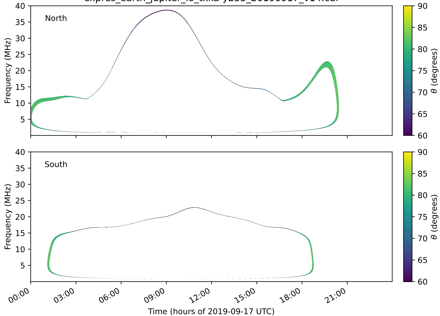
expres_earth_jupiter_io_txka-y235_20190917_v14.cdf
