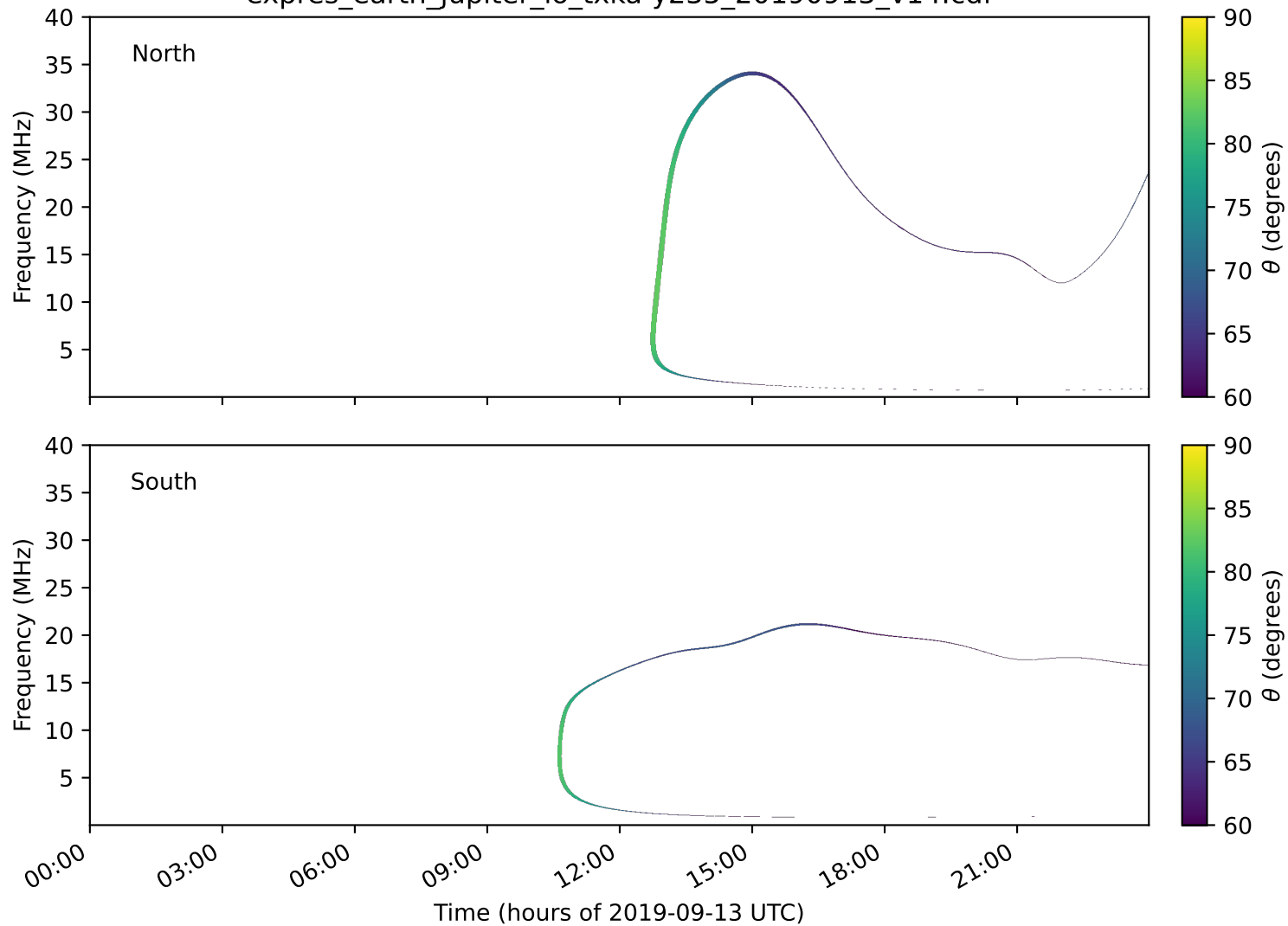
expres_earth_jupiter_io_txka-y235_20190913_v14.cdf
