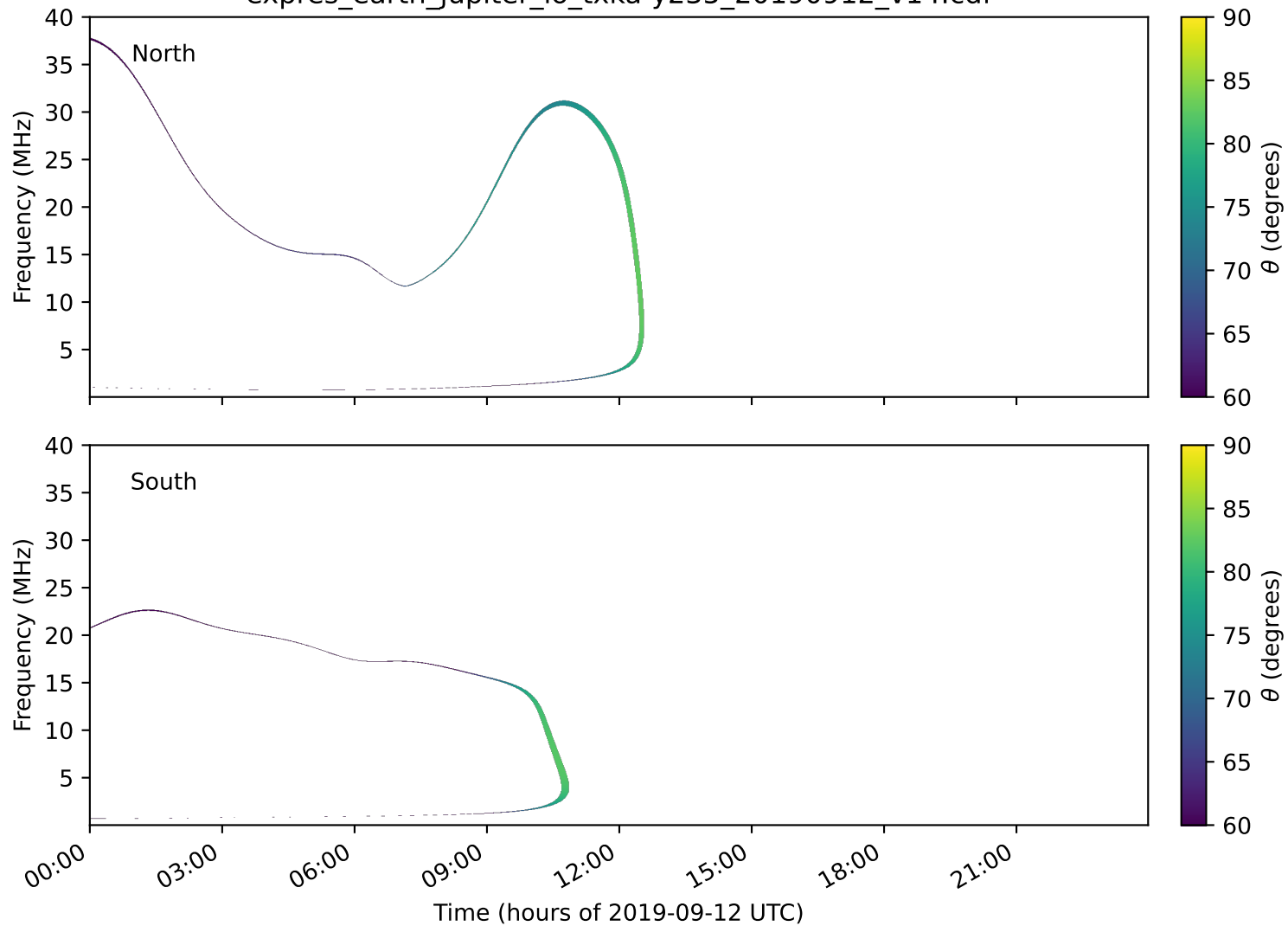
expres_earth_jupiter_io_txka-y235_20190912_v14.cdf
