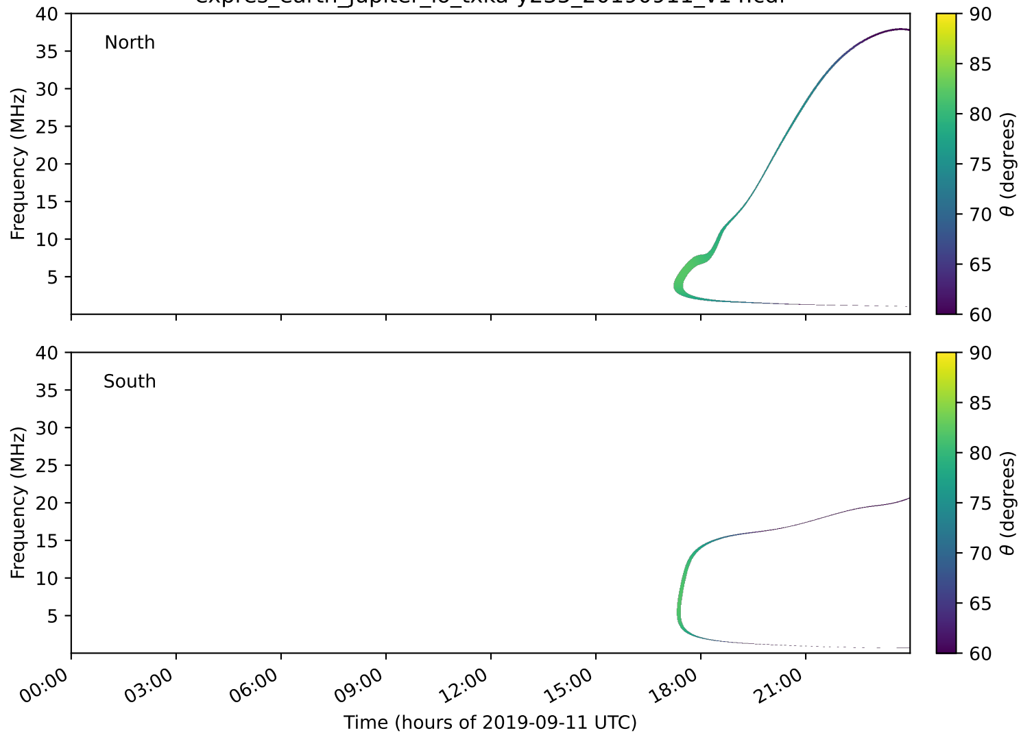
expres_earth_jupiter_io_txka-y235_20190911_v14.cdf
