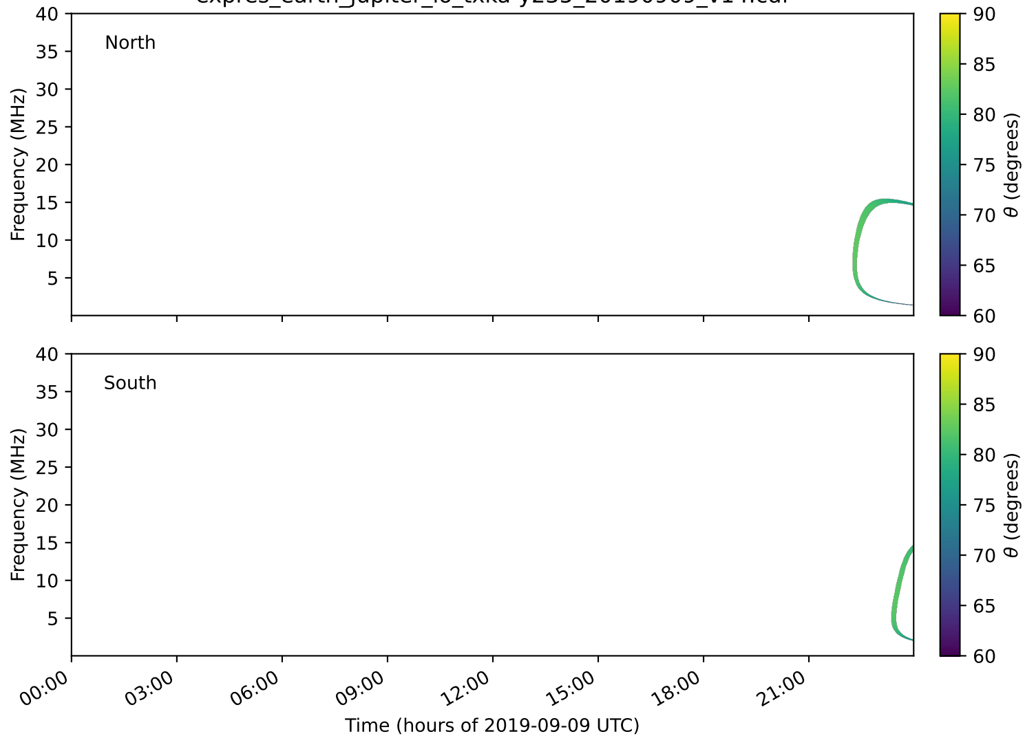
expres_earth_jupiter_io_txka-y235_20190909_v14.cdf
