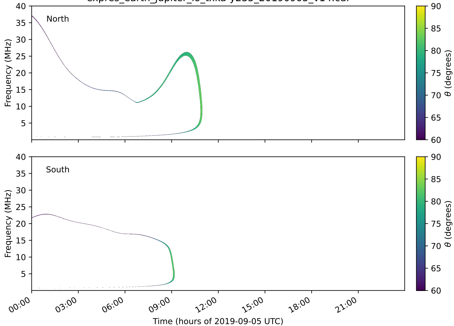
expres_earth_jupiter_io_txka-y235_20190905_v14.cdf
