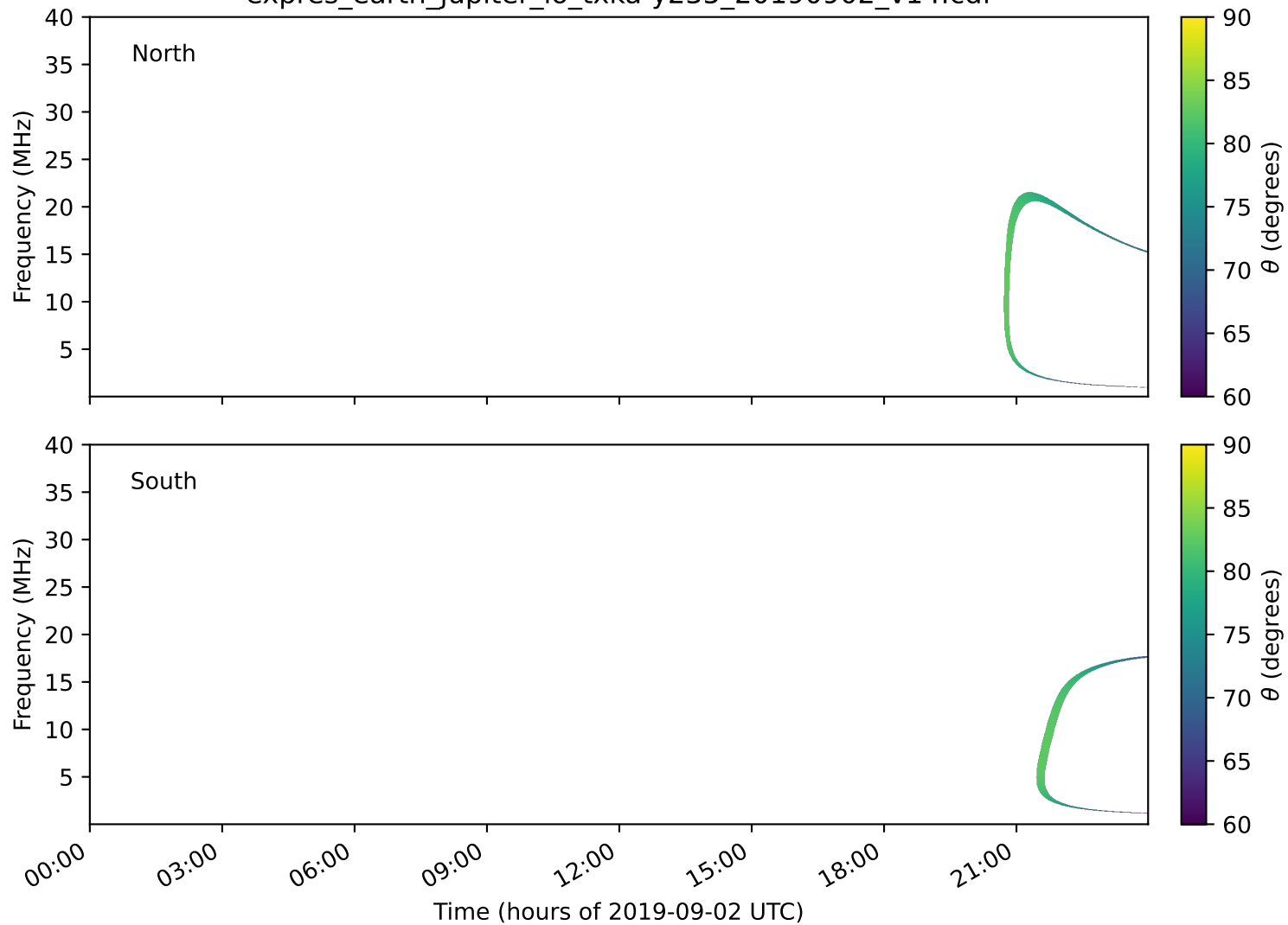
expres_earth_jupiter_io_txka-y235_20190902_v14.cdf
