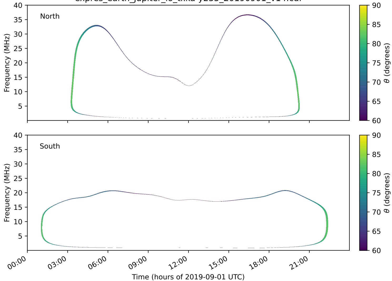
expres_earth_jupiter_io_txka-y235_20190901_v14.cdf
