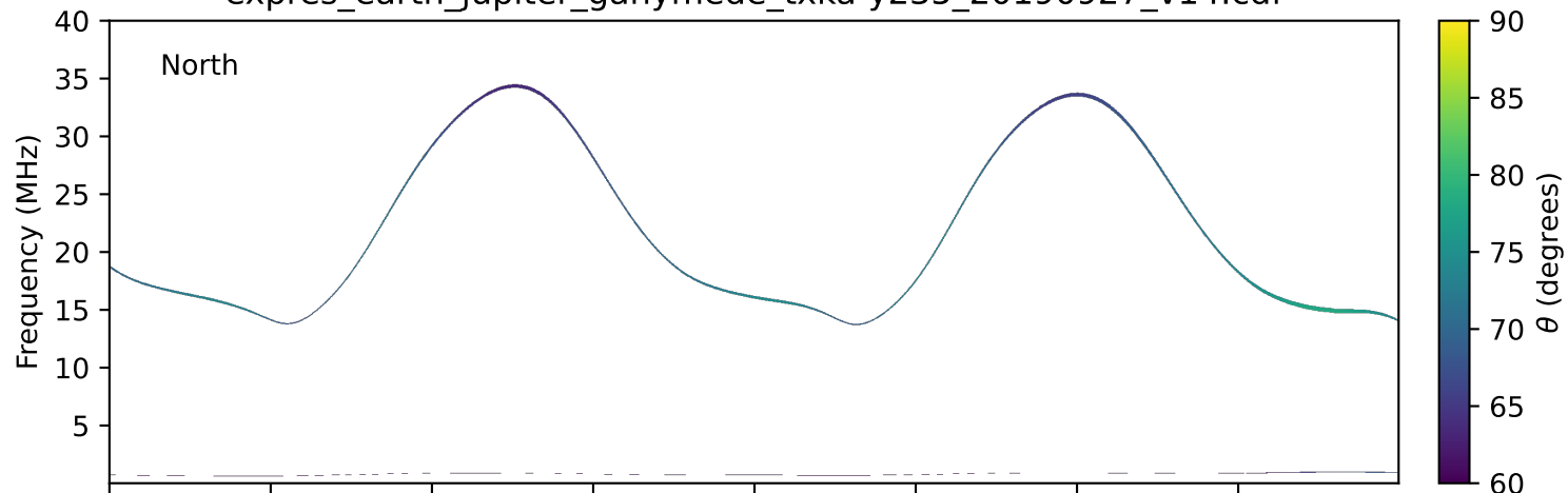
expres_earth_jupiter_ganymede_txka-y235_20190927_v14.cdf
