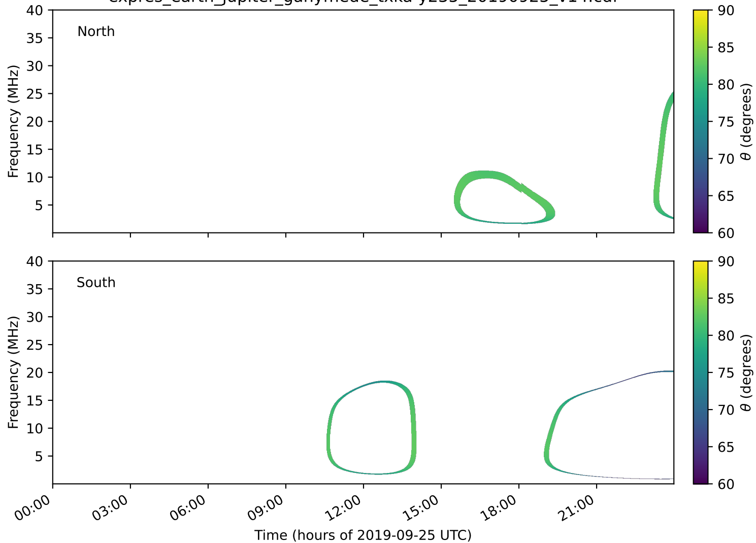
expres_earth_jupiter_ganymede_txka-y235_20190925_v14.cdf
