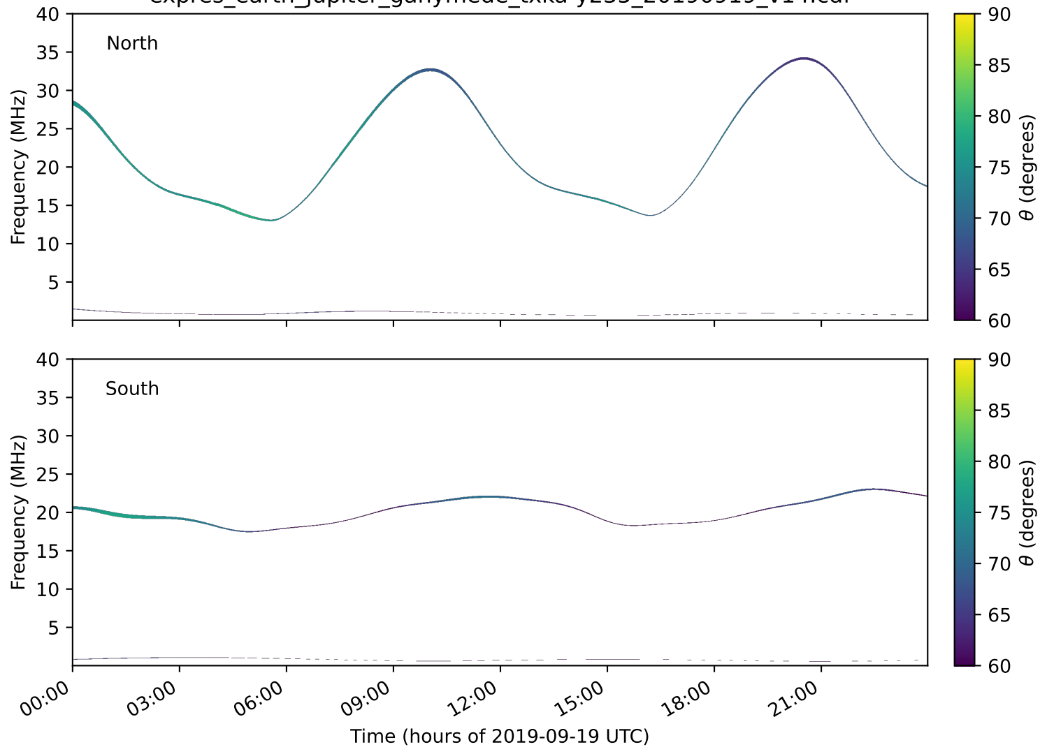
expres_earth_jupiter_ganymede_txka-y235_20190919_v14.cdf
