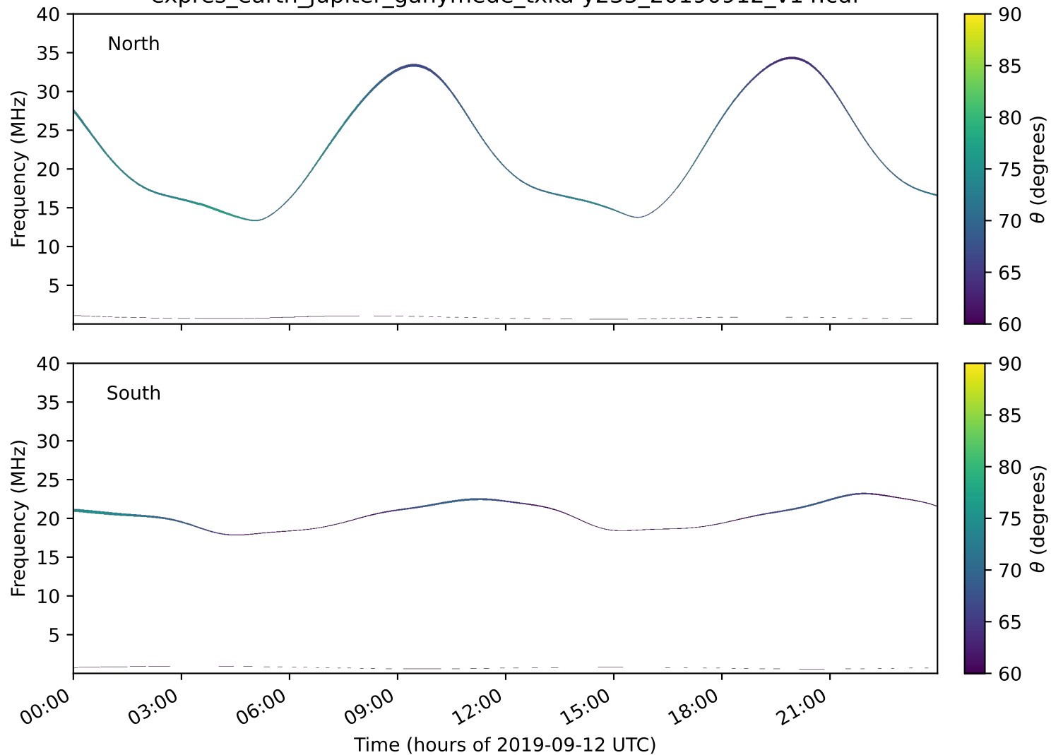
expres_earth_jupiter_ganymede_txka-y235_20190912_v14.cdf
