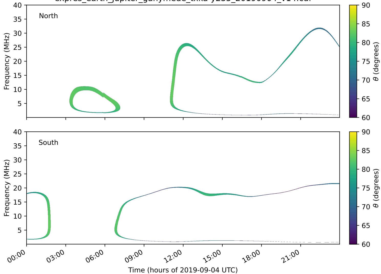
expres_earth_jupiter_ganymede_txka-y235_20190904_v14.cdf
